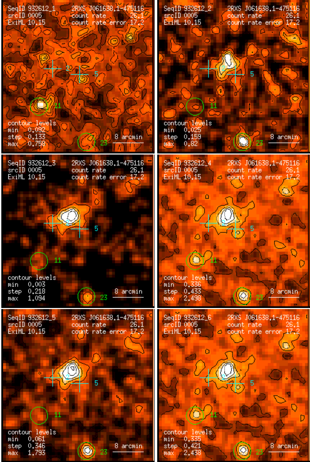
Figure 5: RASS 932612: detection 0005: band rate images, Gaussian filter: (1) PSPC channels 11 – 41, (2) 52 – 90, (3) 91 – 201, (4) 11 – 235, (5) 52 – 201, (6) 11 – 201. Broad band rates in counts/ks. Band rate contour levels in counts/ks/arcmin 2 .
