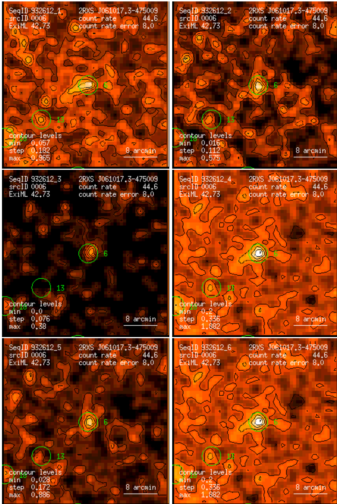
Figure 6: RASS 932612: detection 0006: band rate images, Gaussian filter: (1) PSPC channels 11 – 41, (2) 52 – 90, (3) 91 – 201, (4) 11 – 235, (5) 52 – 201, (6) 11 – 201. Broad band rates in counts/ks. Band rate contour levels in counts/ks/arcmin 2 .
