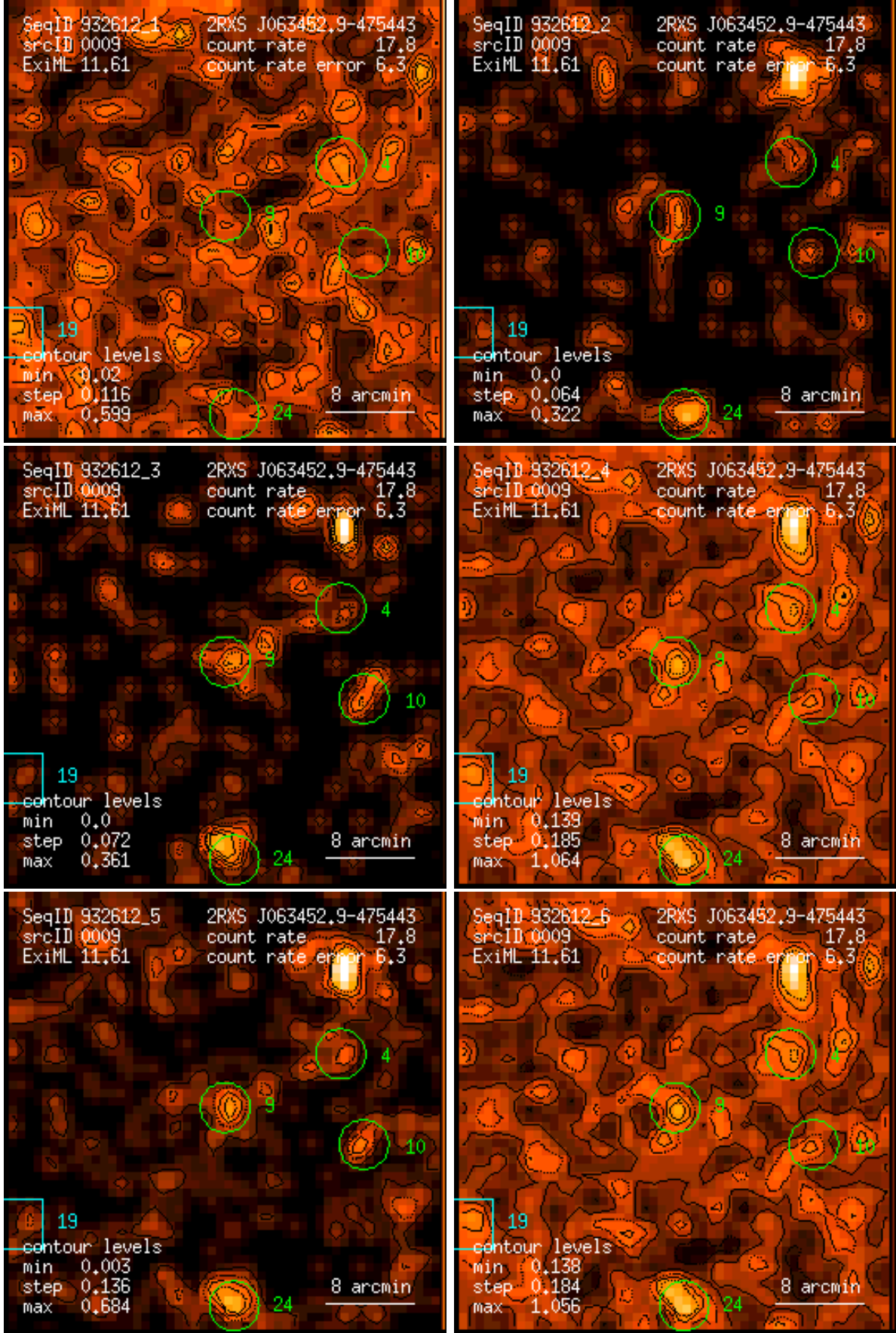
Figure 9: RASS 932612: detection 0009: band rate images, Gaussian filter: (1) PSPC channels 11 – 41, (2) 52 – 90, (3) 91 – 201, (4) 11 – 235, (5) 52 – 201, (6) 11 – 201. Broad band rates in counts/ks. Band rate contour levels in counts/ks/arcmin 2 .
