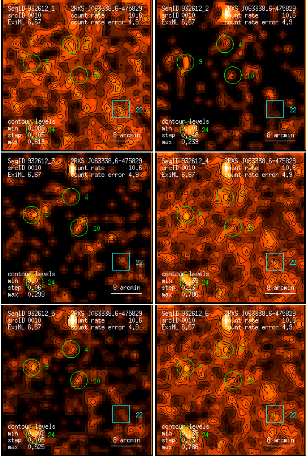
Figure 10: RASS 932612: detection 0010: band rate images, Gaussian filter: (1) PSPC channels 11 – 41, (2) 52 – 90, (3) 91 – 201, (4) 11 – 235, (5) 52 – 201, (6) 11 – 201. Broad band rates in counts/ks. Band rate contour levels in counts/ks/arcmin 2 .
