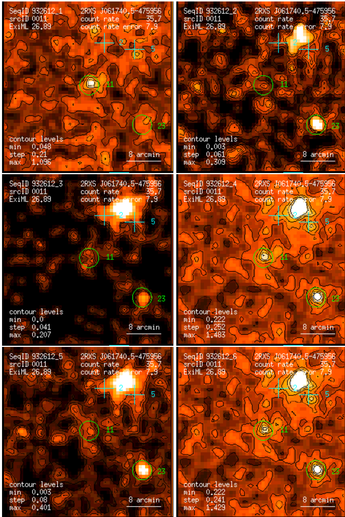
Figure 11: RASS 932612: detection 0011: band rate images, Gaussian filter: (1) PSPC channels 11 – 41, (2) 52 – 90, (3) 91 – 201, (4) 11 – 235, (5) 52 – 201, (6) 11 – 201. Broad band rates in counts/ks. Band rate contour levels in counts/ks/arcmin 2 .
