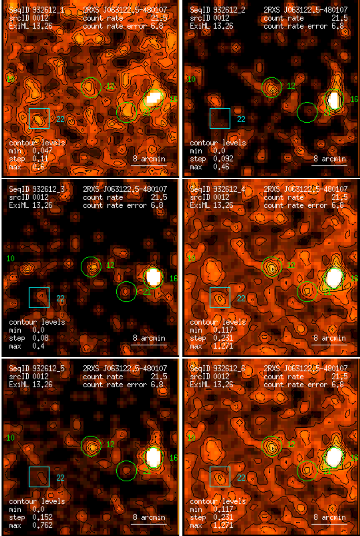
Figure 12: RASS 932612: detection 0012: band rate images, Gaussian filter: (1) PSPC channels 11 – 41, (2) 52 – 90, (3) 91 – 201, (4) 11 – 235, (5) 52 – 201, (6) 11 – 201. Broad band rates in counts/ks. Band rate contour levels in counts/ks/arcmin 2 .
