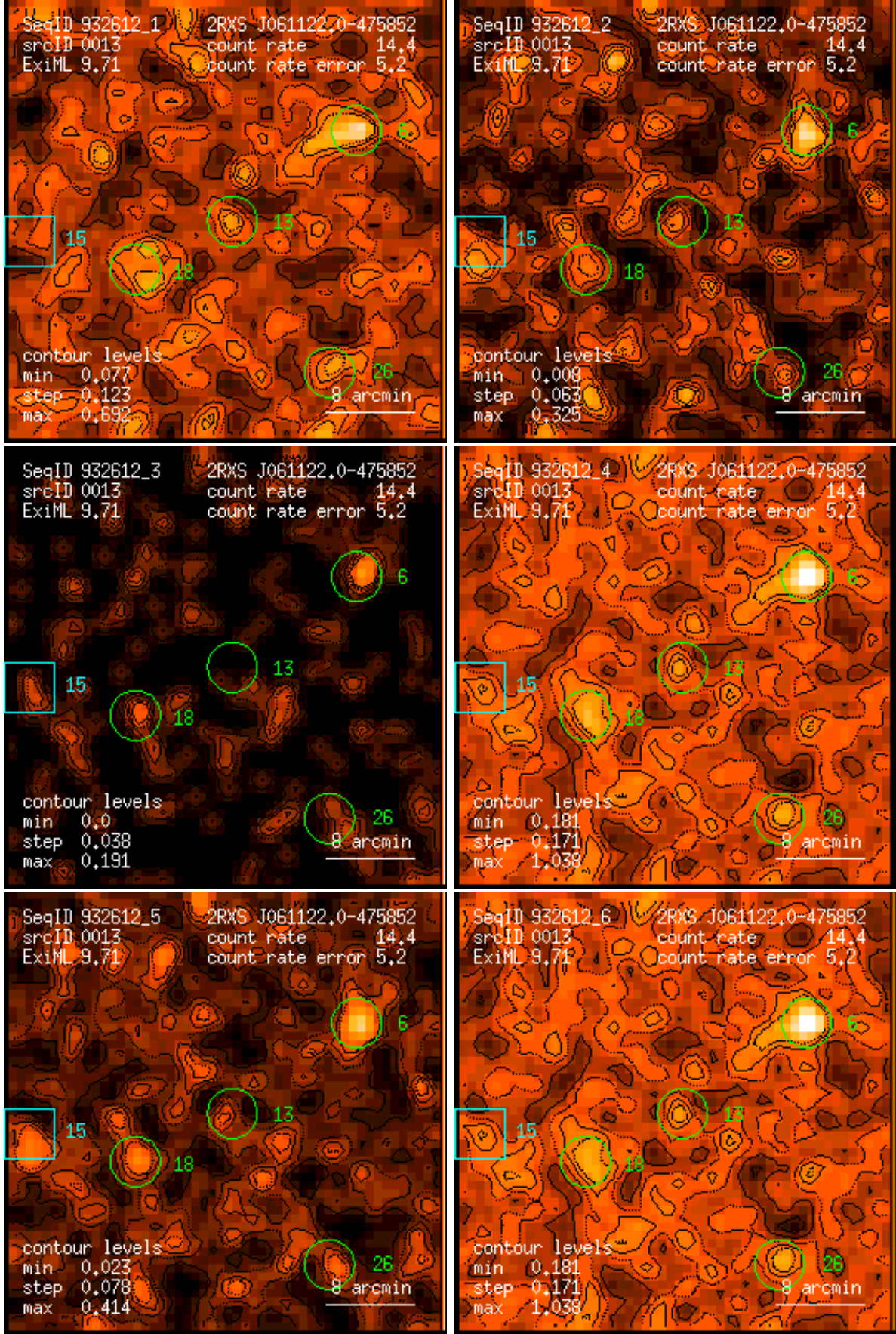
Figure 13: RASS 932612: detection 0013: band rate images, Gaussian filter: (1) PSPC channels 11 – 41, (2) 52 – 90, (3) 91 – 201, (4) 11 – 235, (5) 52 – 201, (6) 11 – 201. Broad band rates in counts/ks. Band rate contour levels in counts/ks/arcmin 2 .
