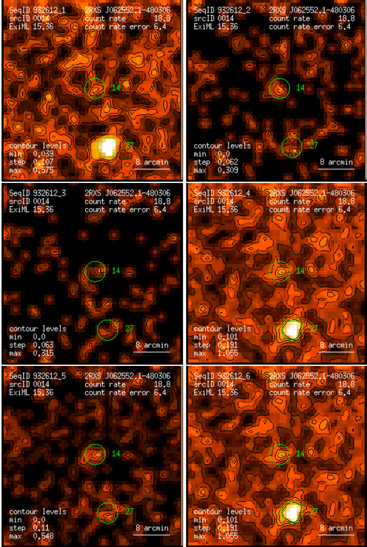
Figure 14: RASS 932612: detection 0014: band rate images, Gaussian filter: (1) PSPC channels 11 – 41, (2) 52 – 90, (3) 91 – 201, (4) 11 – 235, (5) 52 – 201, (6) 11 – 201. Broad band rates in counts/ks. Band rate contour levels in counts/ks/arcmin 2 .
