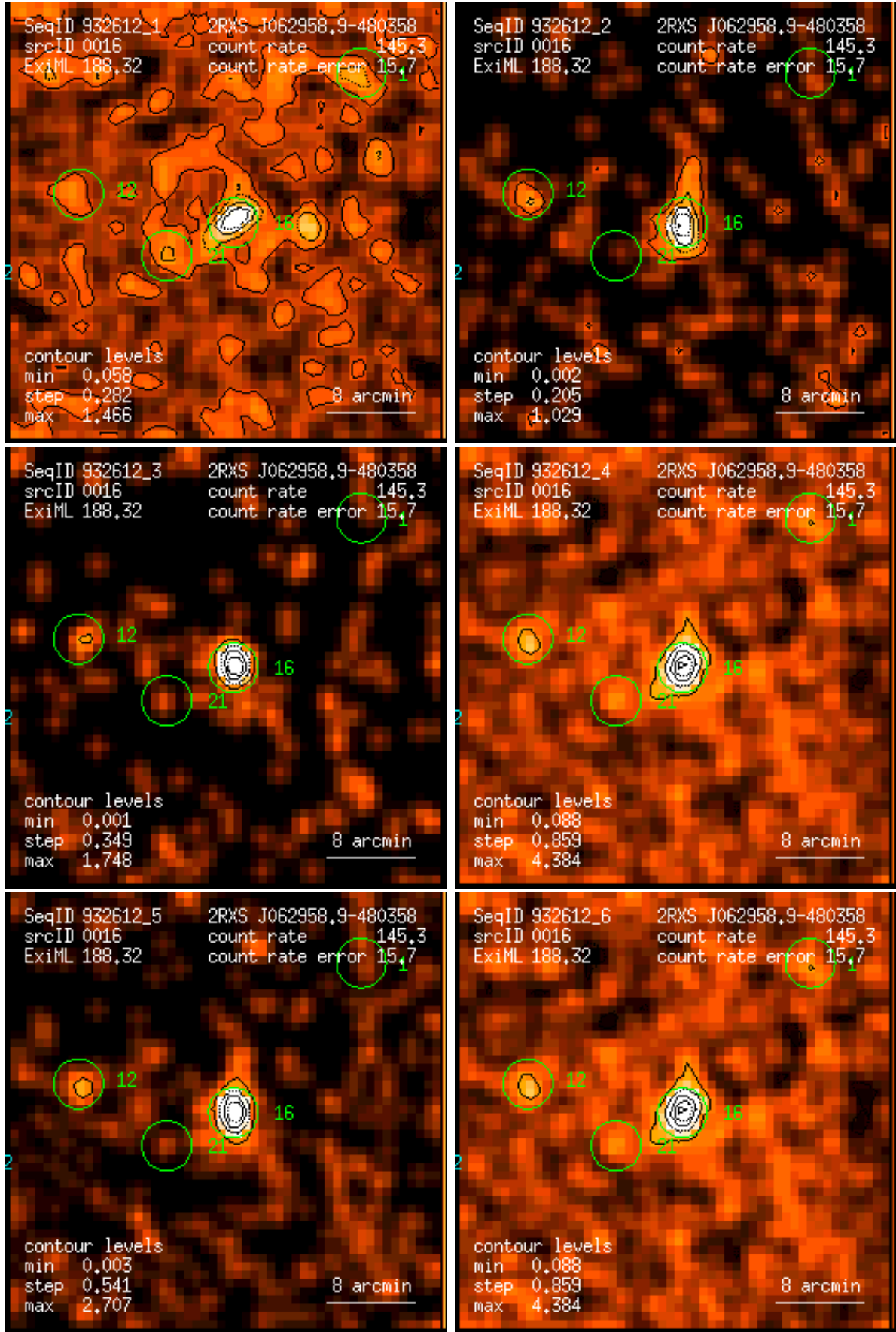
Figure 16: RASS 932612: detection 0016: band rate images, Gaussian filter: (1) PSPC channels 11 – 41, (2) 52 – 90, (3) 91 – 201, (4) 11 – 235, (5) 52 – 201, (6) 11 – 201. Broad band rates in counts/ks. Band rate contour levels in counts/ks/arcmin 2 .
