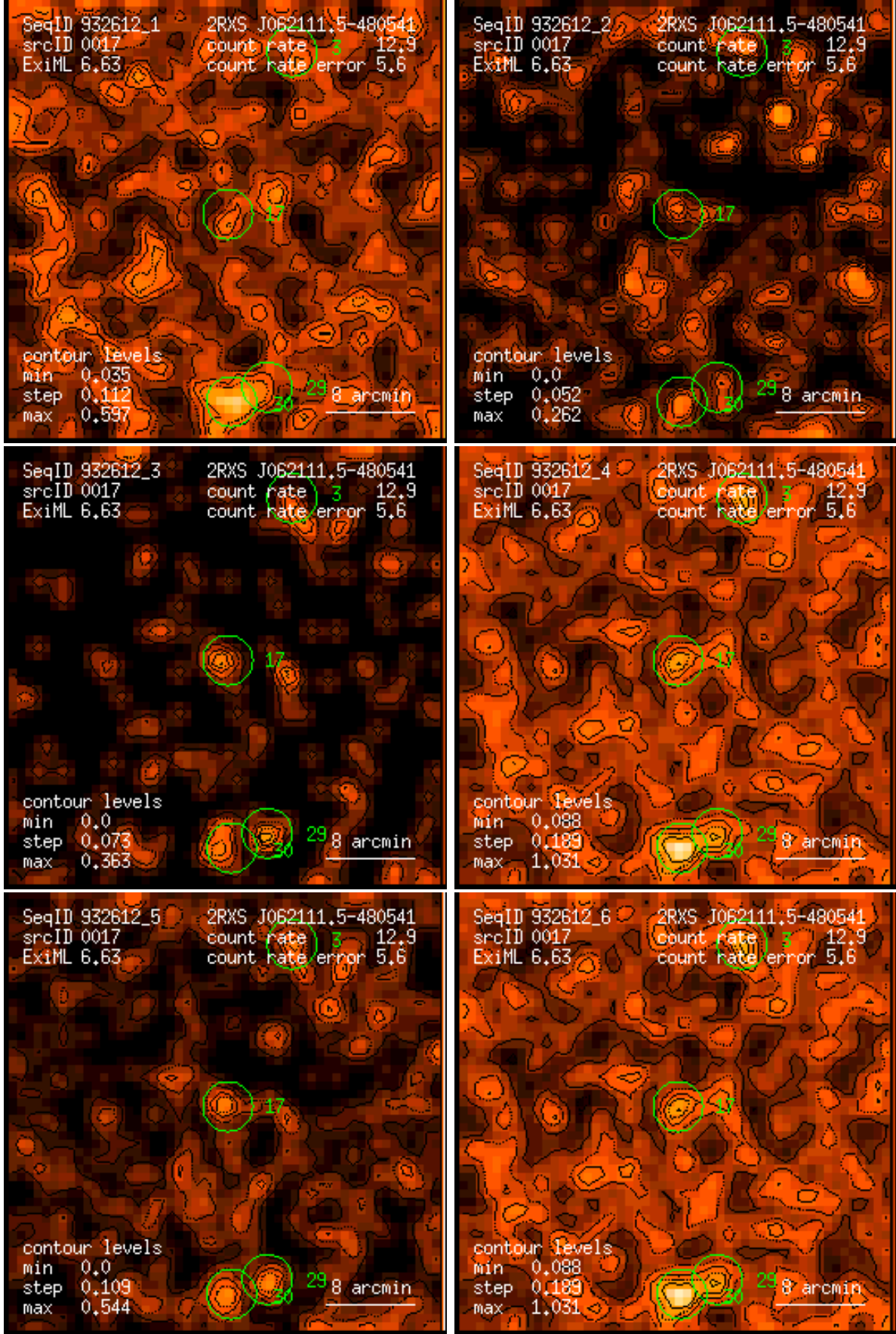
Figure 17: RASS 932612: detection 0017: band rate images, Gaussian filter: (1) PSPC channels 11 – 41, (2) 52 – 90, (3) 91 – 201, (4) 11 – 235, (5) 52 – 201, (6) 11 – 201. Broad band rates in counts/ks. Band rate contour levels in counts/ks/arcmin 2 .
