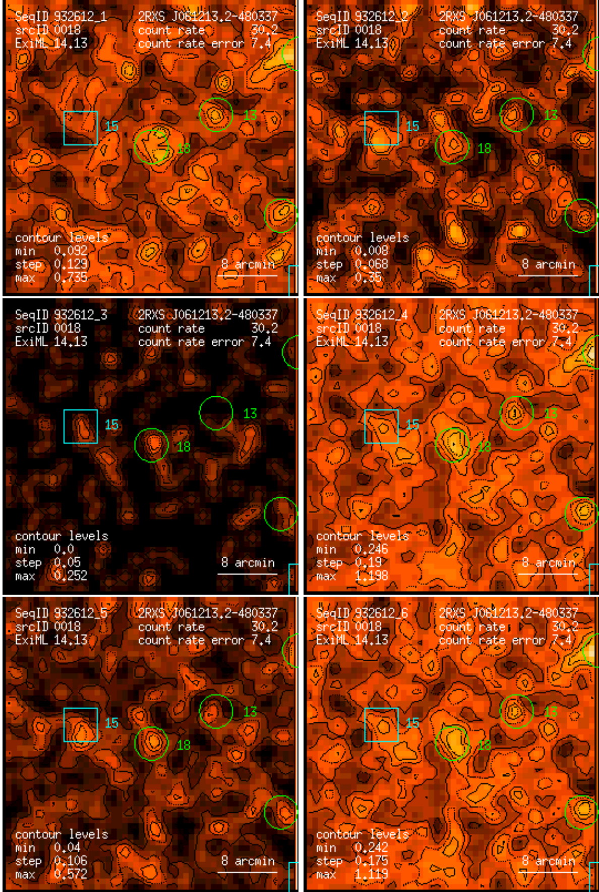
Figure 18: RASS 932612: detection 0018: band rate images, Gaussian filter: (1) PSPC channels 11 – 41, (2) 52 – 90, (3) 91 – 201, (4) 11 – 235, (5) 52 – 201, (6) 11 – 201. Broad band rates in counts/ks. Band rate contour levels in counts/ks/arcmin 2 .
