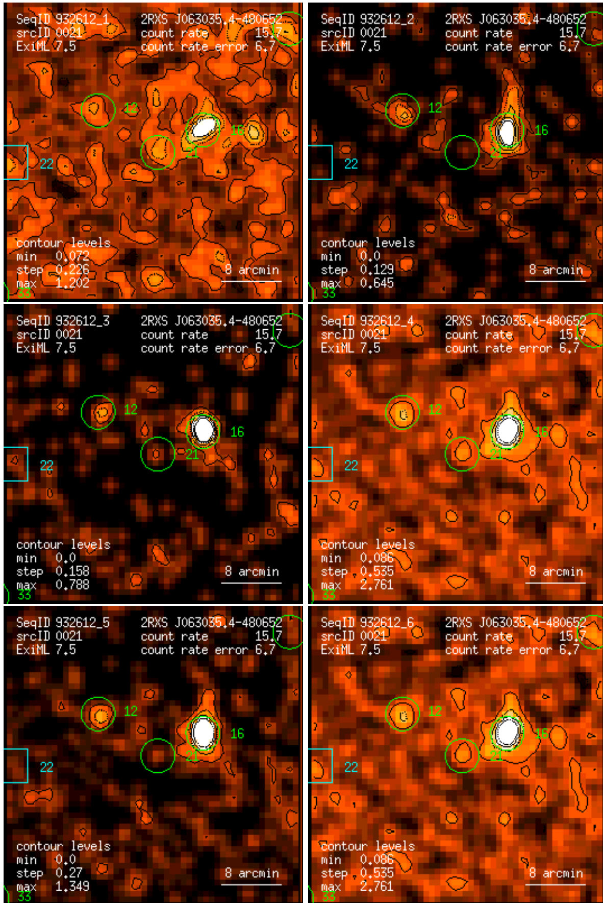
Figure 21: RASS 932612: detection 0021: band rate images, Gaussian filter: (1) PSPC channels 11 – 41, (2) 52 – 90, (3) 91 – 201, (4) 11 – 235, (5) 52 – 201, (6) 11 – 201. Broad band rates in counts/ks. Band rate contour levels in counts/ks/arcmin 2 .
