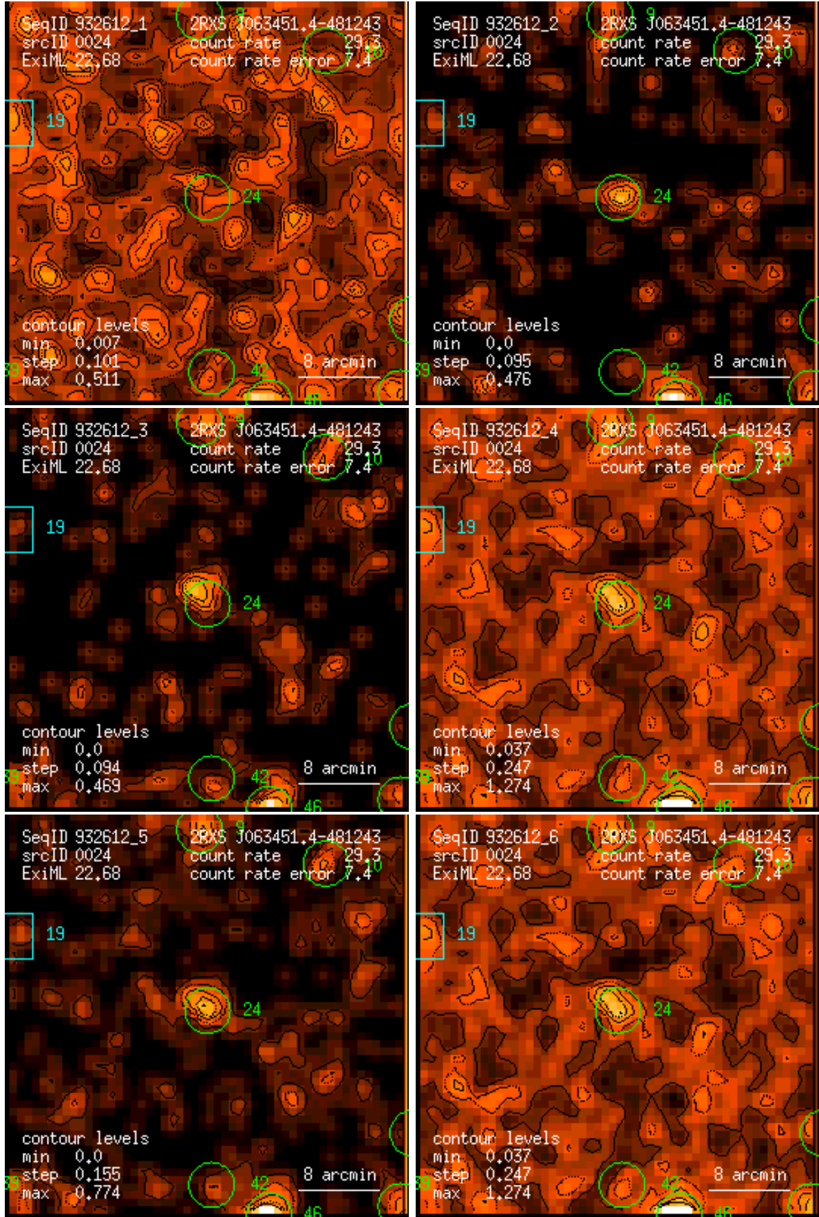
Figure 24: RASS 932612: detection 0024: band rate images, Gaussian filter: (1) PSPC channels 11 – 41, (2) 52 – 90, (3) 91 – 201, (4) 11 – 235, (5) 52 – 201, (6) 11 – 201. Broad band rates in counts/ks. Band rate contour levels in counts/ks/arcmin 2 .
