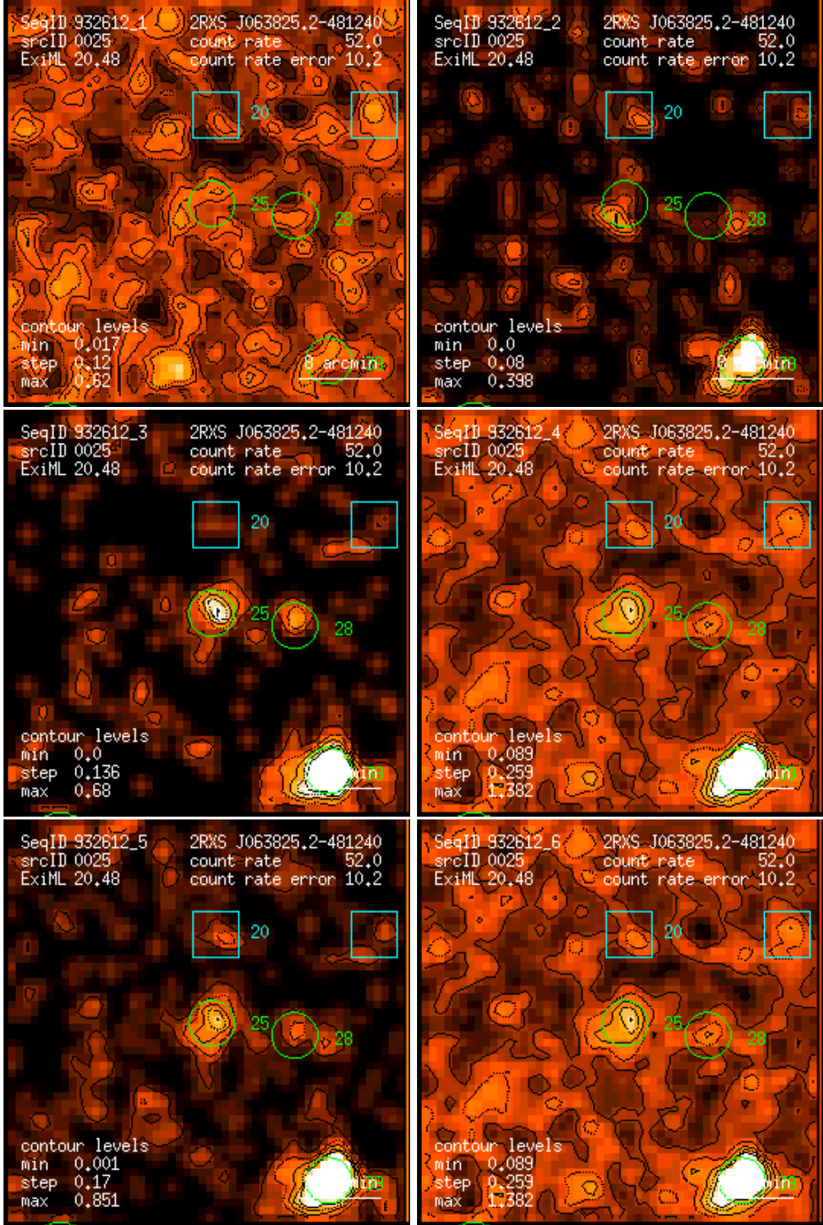
Figure 25: RASS 932612: detection 0025: band rate images, Gaussian filter: (1) PSPC channels 11 – 41, (2) 52 – 90, (3) 91 – 201, (4) 11 – 235, (5) 52 – 201, (6) 11 – 201. Broad band rates in counts/ks. Band rate contour levels in counts/ks/arcmin 2 .
