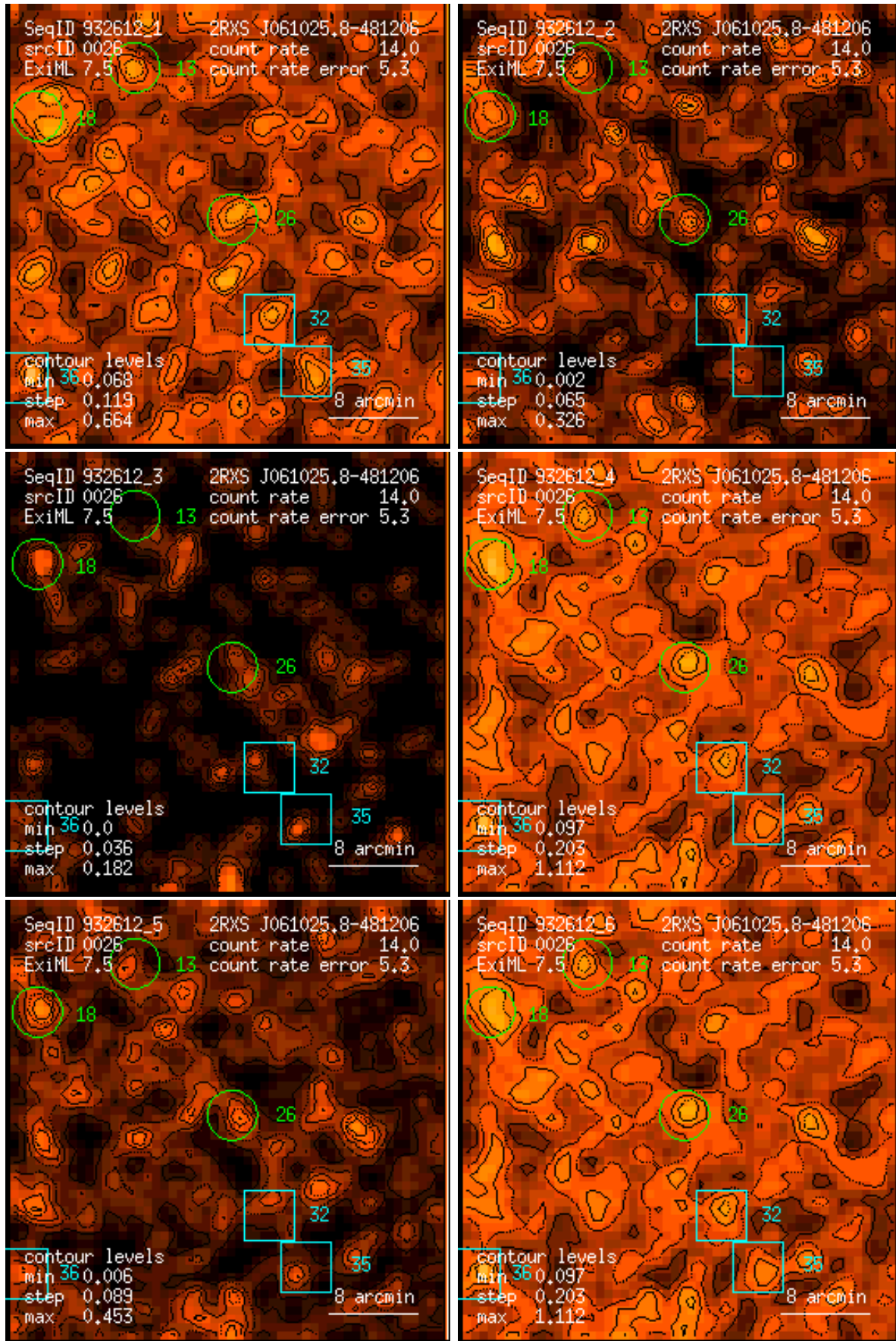
Figure 26: RASS 932612: detection 0026: band rate images, Gaussian filter: (1) PSPC channels 11 – 41, (2) 52 – 90, (3) 91 – 201, (4) 11 – 235, (5) 52 – 201, (6) 11 – 201. Broad band rates in counts/ks. Band rate contour levels in counts/ks/arcmin 2 .
