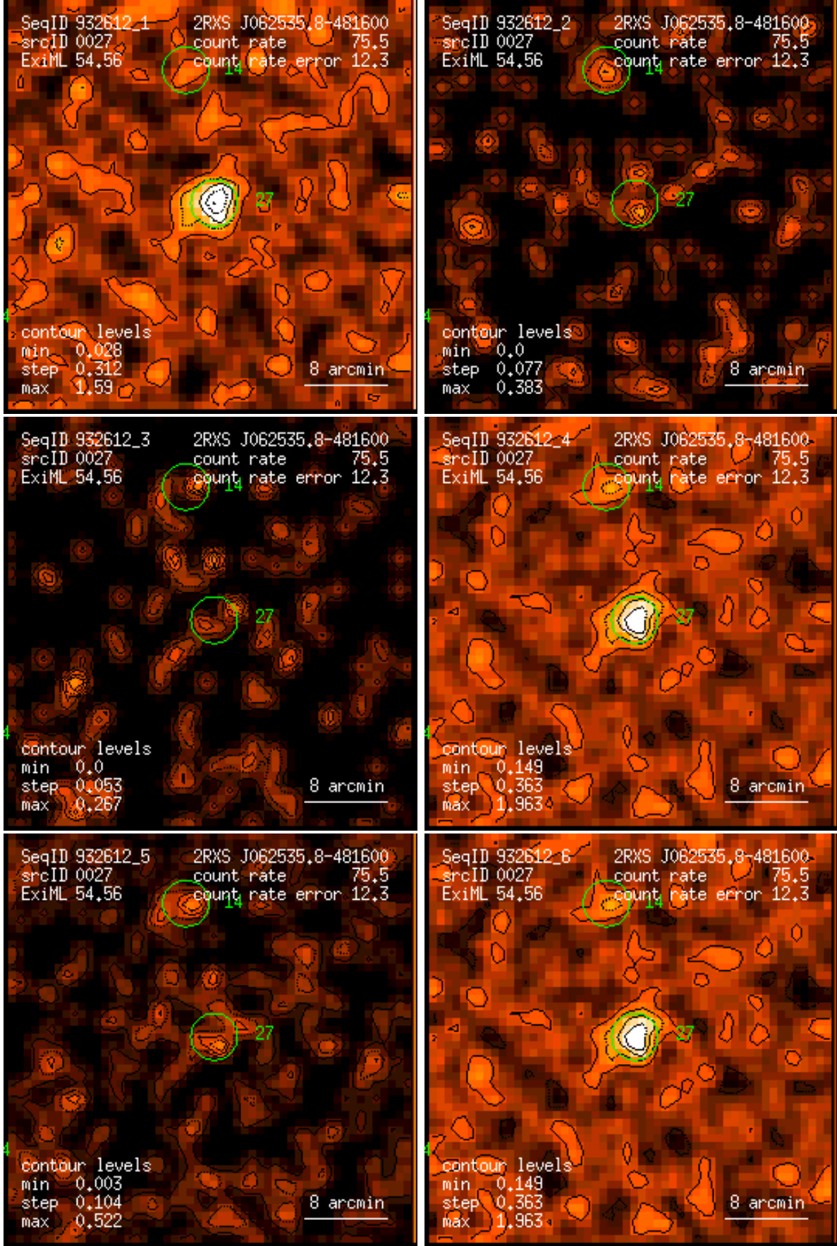
Figure 27: RASS 932612: detection 0027: band rate images, Gaussian filter: (1) PSPC channels 11 – 41, (2) 52 – 90, (3) 91 – 201, (4) 11 – 235, (5) 52 – 201, (6) 11 – 201. Broad band rates in counts/ks. Band rate contour levels in counts/ks/arcmin 2 .
