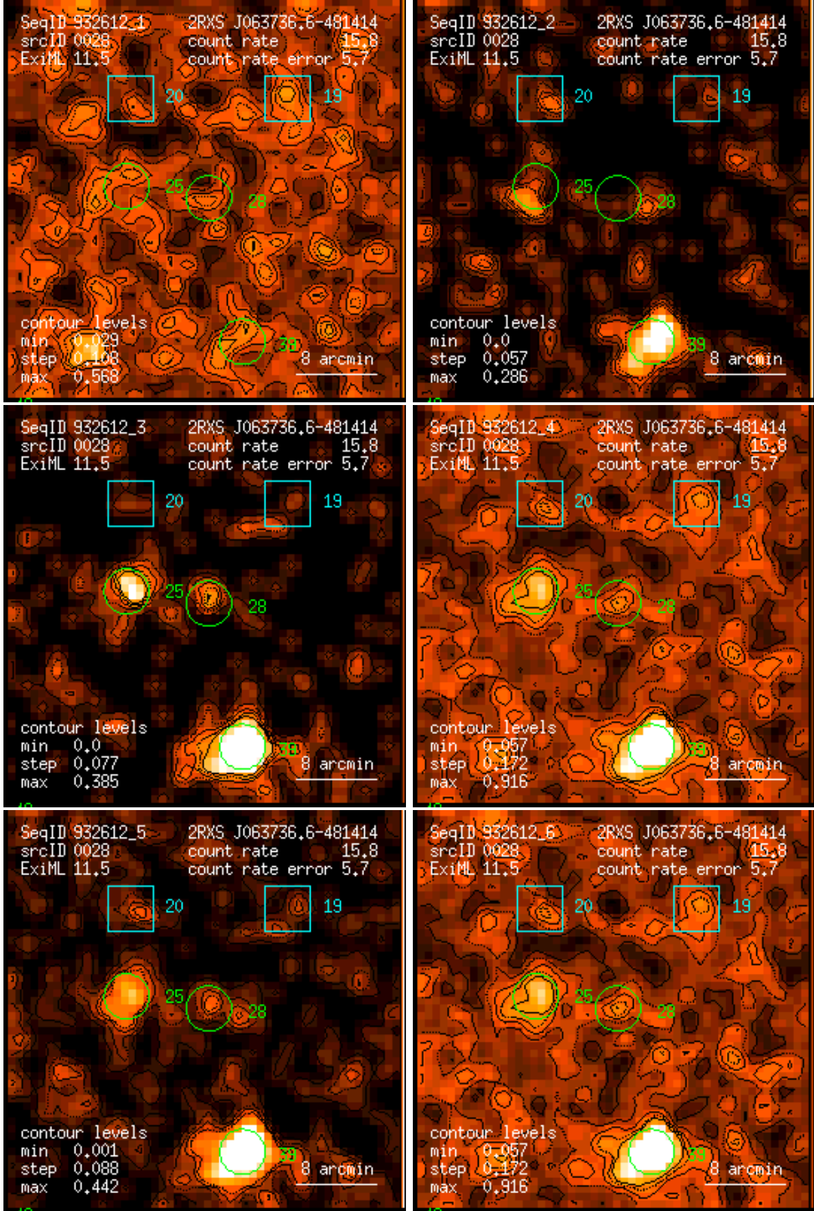
Figure 28: RASS 932612: detection 0028: band rate images, Gaussian filter: (1) PSPC channels 11 – 41, (2) 52 – 90, (3) 91 – 201, (4) 11 – 235, (5) 52 – 201, (6) 11 – 201. Broad band rates in counts/ks. Band rate contour levels in counts/ks/arcmin 2 .
