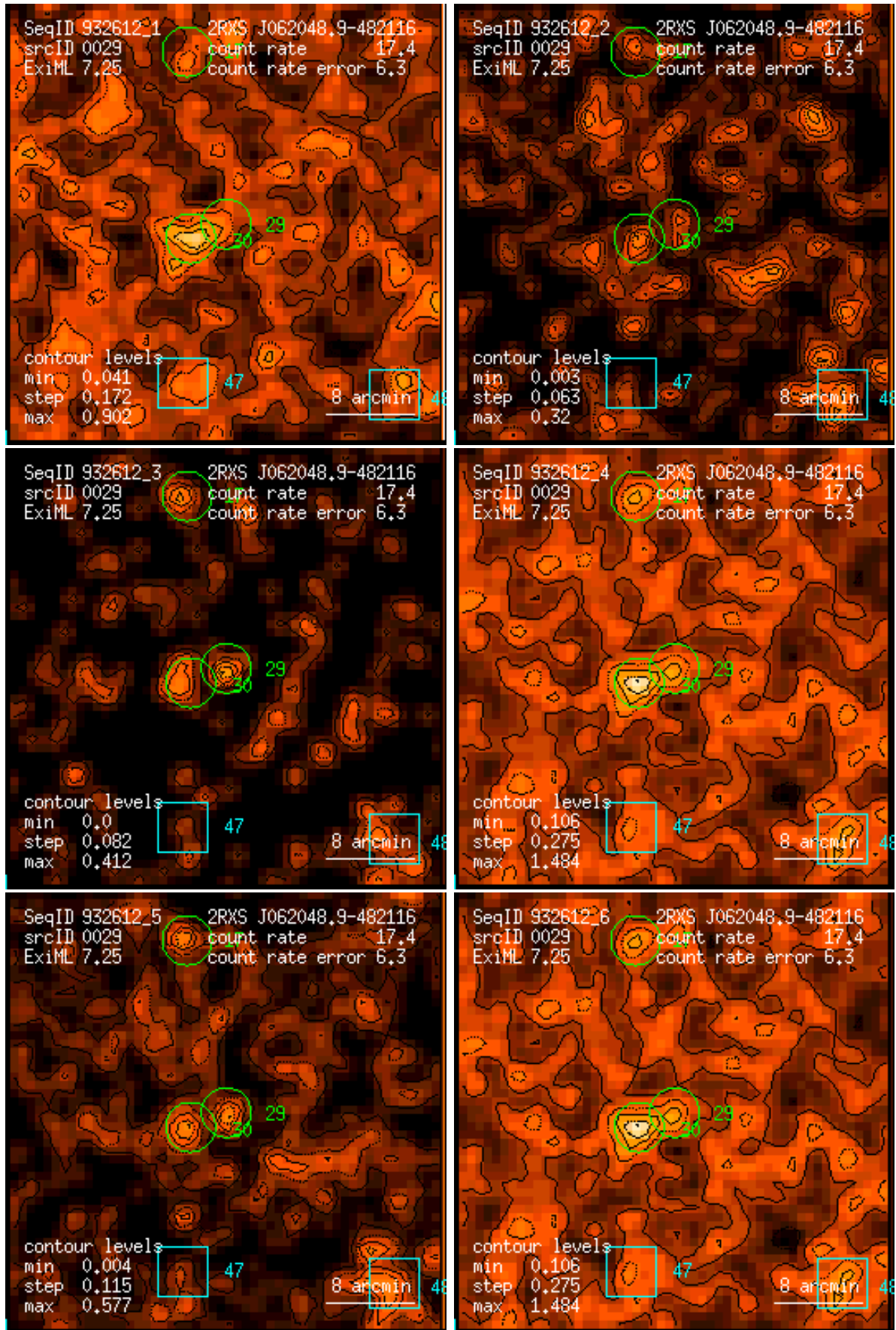
Figure 29: RASS 932612: detection 0029: band rate images, Gaussian filter: (1) PSPC channels 11 – 41, (2) 52 – 90, (3) 91 – 201, (4) 11 – 235, (5) 52 – 201, (6) 11 – 201. Broad band rates in counts/ks. Band rate contour levels in counts/ks/arcmin 2 .
