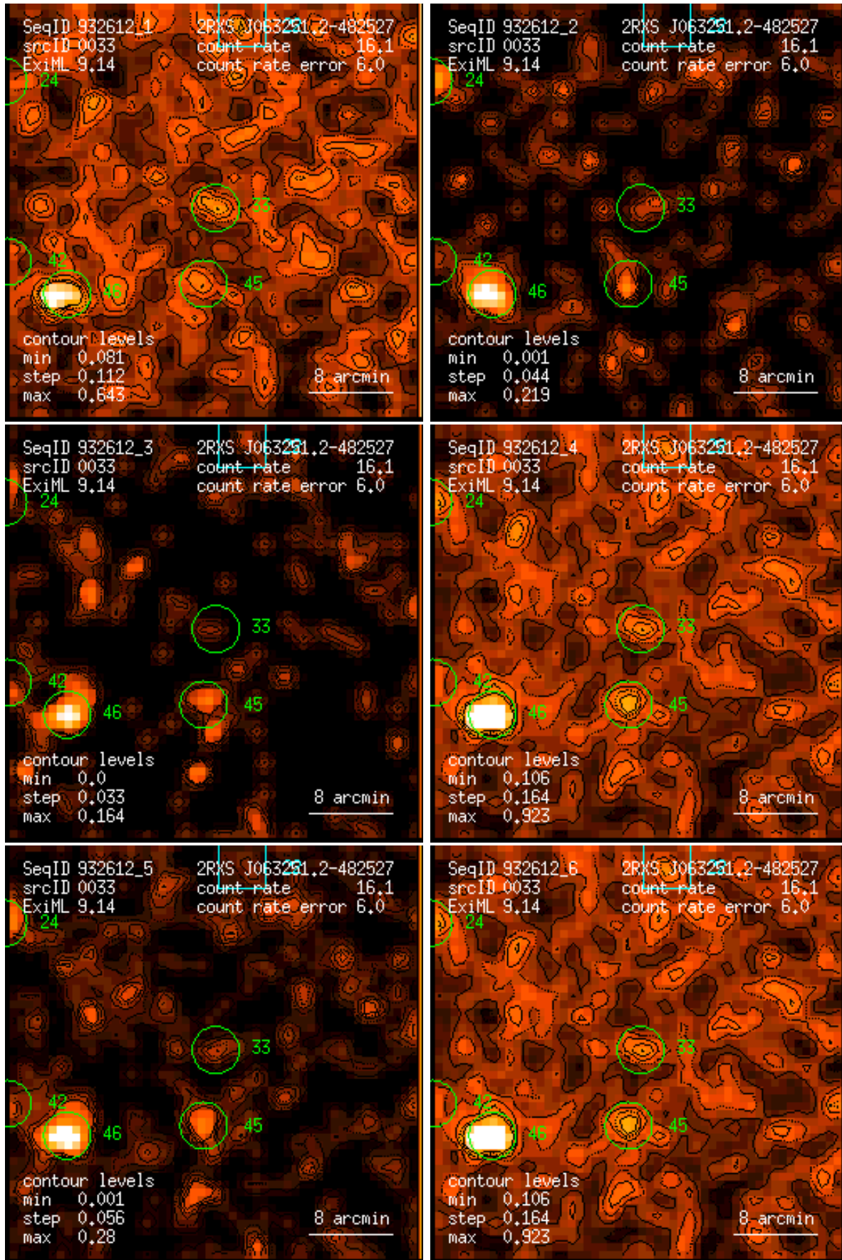
Figure 33: RASS 932612: detection 0033: band rate images, Gaussian filter: (1) PSPC channels 11 – 41, (2) 52 – 90, (3) 91 – 201, (4) 11 – 235, (5) 52 – 201, (6) 11 – 201. Broad band rates in counts/ks. Band rate contour levels in counts/ks/arcmin 2 .
