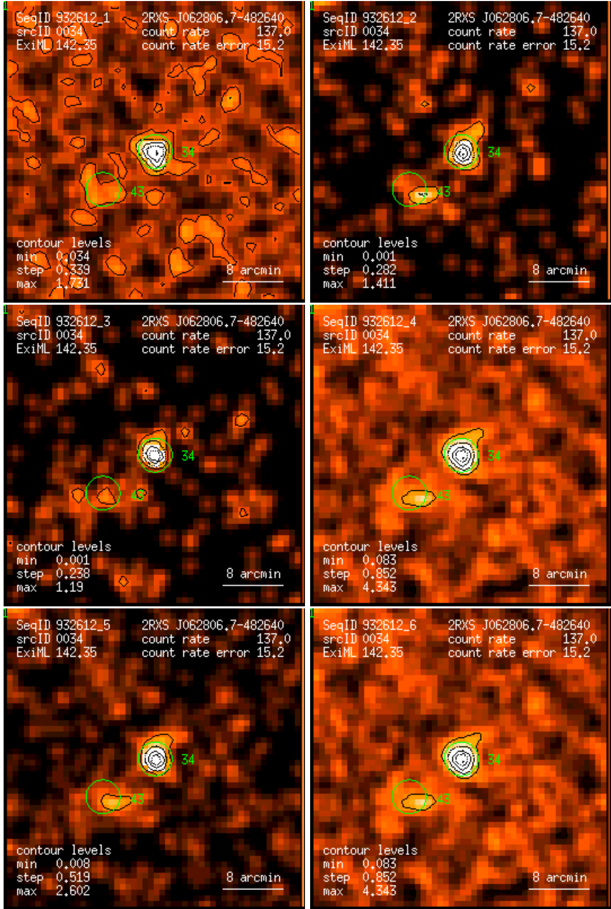
Figure 34: RASS 932612: detection 0034: band rate images, Gaussian filter: (1) PSPC channels 11 – 41, (2) 52 – 90, (3) 91 – 201, (4) 11 – 235, (5) 52 – 201, (6) 11 – 201. Broad band rates in counts/ks. Band rate contour levels in counts/ks/arcmin 2 .
