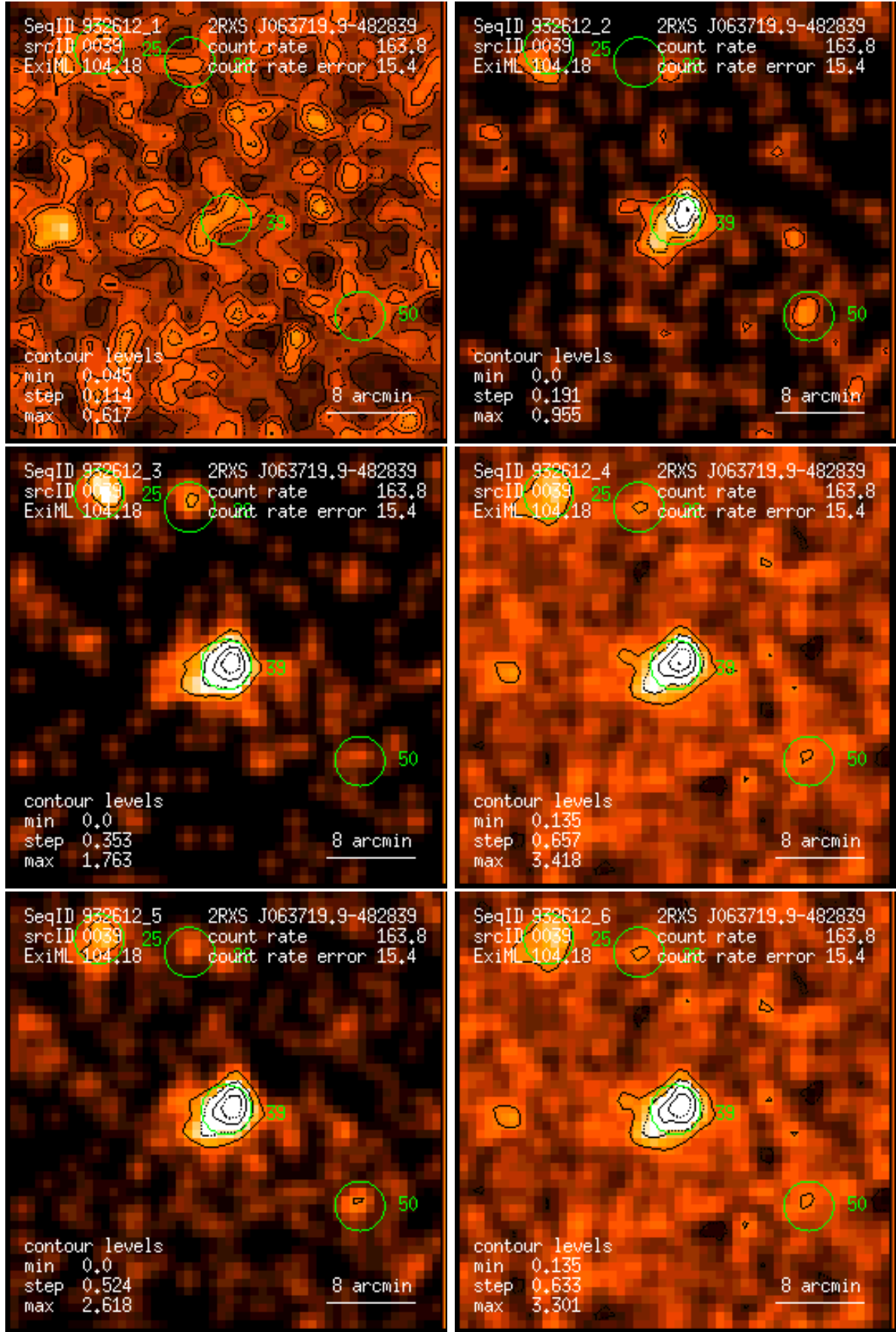
Figure 39: RASS 932612: detection 0039: band rate images, Gaussian filter: (1) PSPC channels 11 – 41, (2) 52 – 90, (3) 91 – 201, (4) 11 – 235, (5) 52 – 201, (6) 11 – 201. Broad band rates in counts/ks. Band rate contour levels in counts/ks/arcmin 2 .
