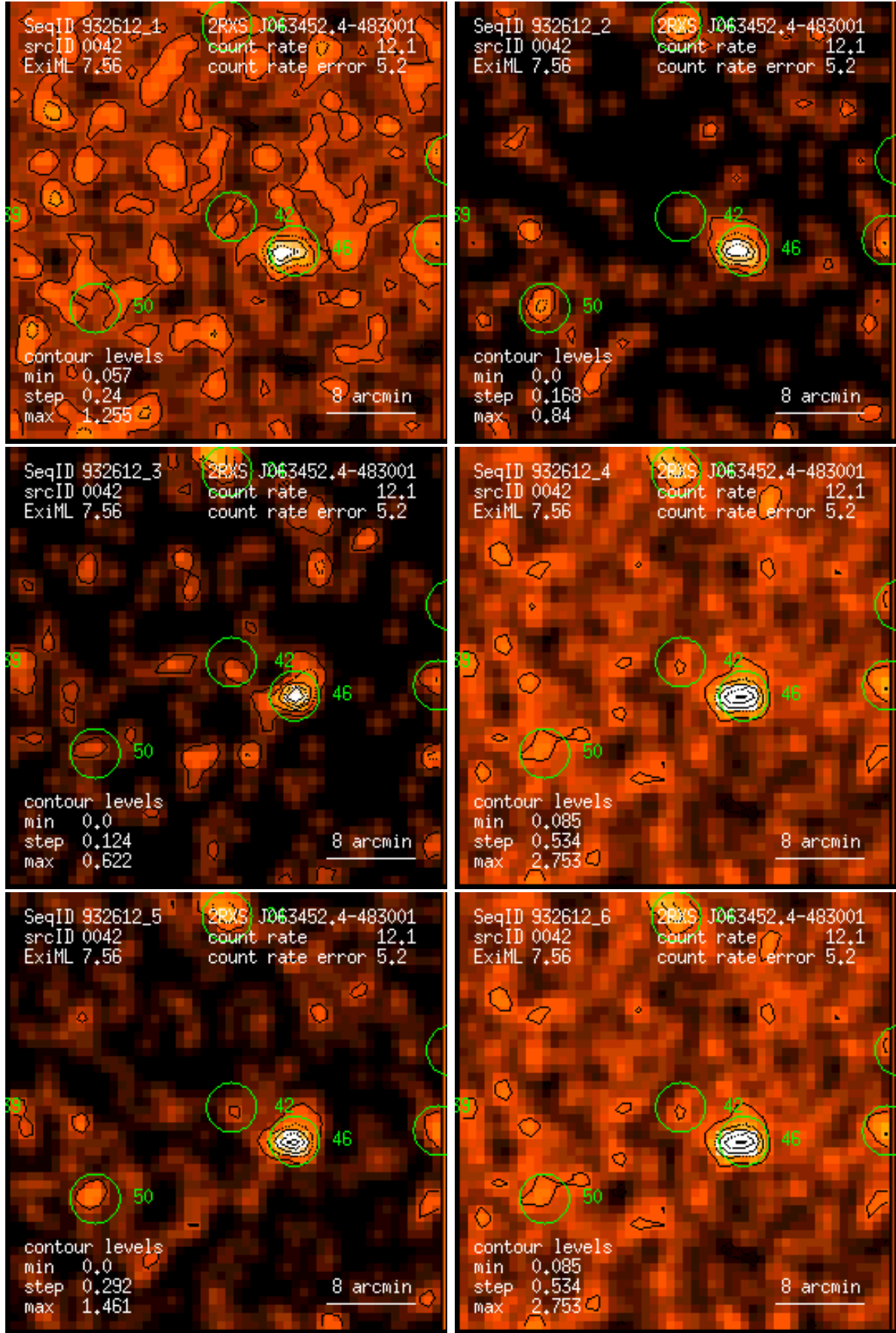
Figure 42: RASS 932612: detection 0042: band rate images, Gaussian filter: (1) PSPC channels 11 – 41, (2) 52 – 90, (3) 91 – 201, (4) 11 – 235, (5) 52 – 201, (6) 11 – 201. Broad band rates in counts/ks. Band rate contour levels in counts/ks/arcmin 2 .
