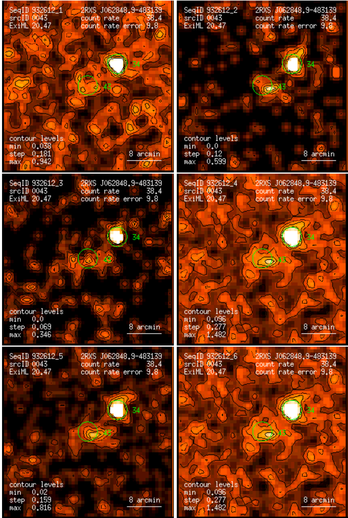
Figure 43: RASS 932612: detection 0043: band rate images, Gaussian filter: (1) PSPC channels 11 – 41, (2) 52 – 90, (3) 91 – 201, (4) 11 – 235, (5) 52 – 201, (6) 11 – 201. Broad band rates in counts/ks. Band rate contour levels in counts/ks/arcmin 2 .
