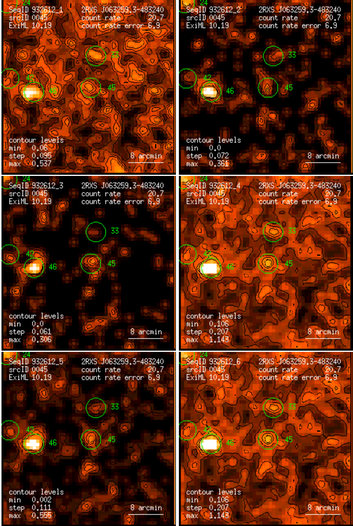
Figure 45: RASS 932612: detection 0045: band rate images, Gaussian filter: (1) PSPC channels 11 – 41, (2) 52 – 90, (3) 91 – 201, (4) 11 – 235, (5) 52 – 201, (6) 11 – 201. Broad band rates in counts/ks. Band rate contour levels in counts/ks/arcmin 2 .
