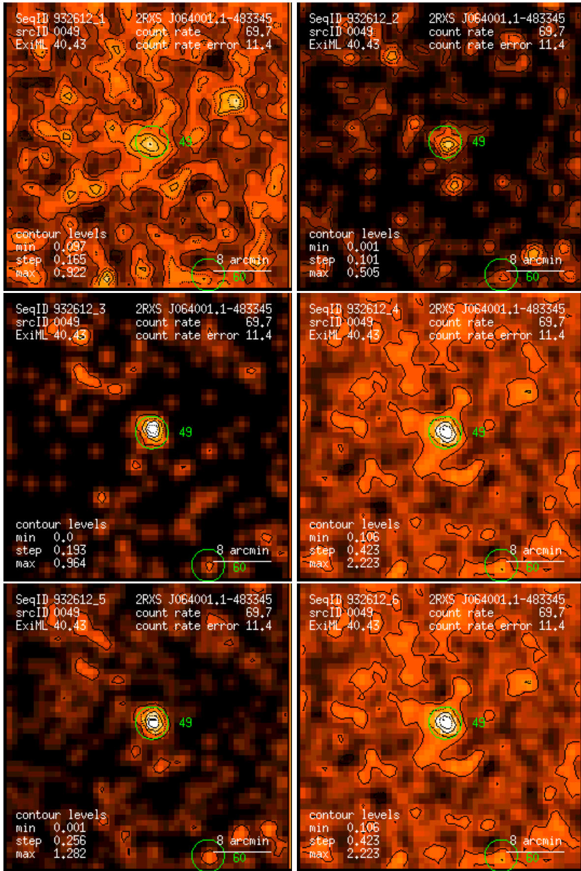
Figure 49: RASS 932612: detection 0049: band rate images, Gaussian filter: (1) PSPC channels 11 – 41, (2) 52 – 90, (3) 91 – 201, (4) 11 – 235, (5) 52 – 201, (6) 11 – 201. Broad band rates in counts/ks. Band rate contour levels in counts/ks/arcmin 2 .
