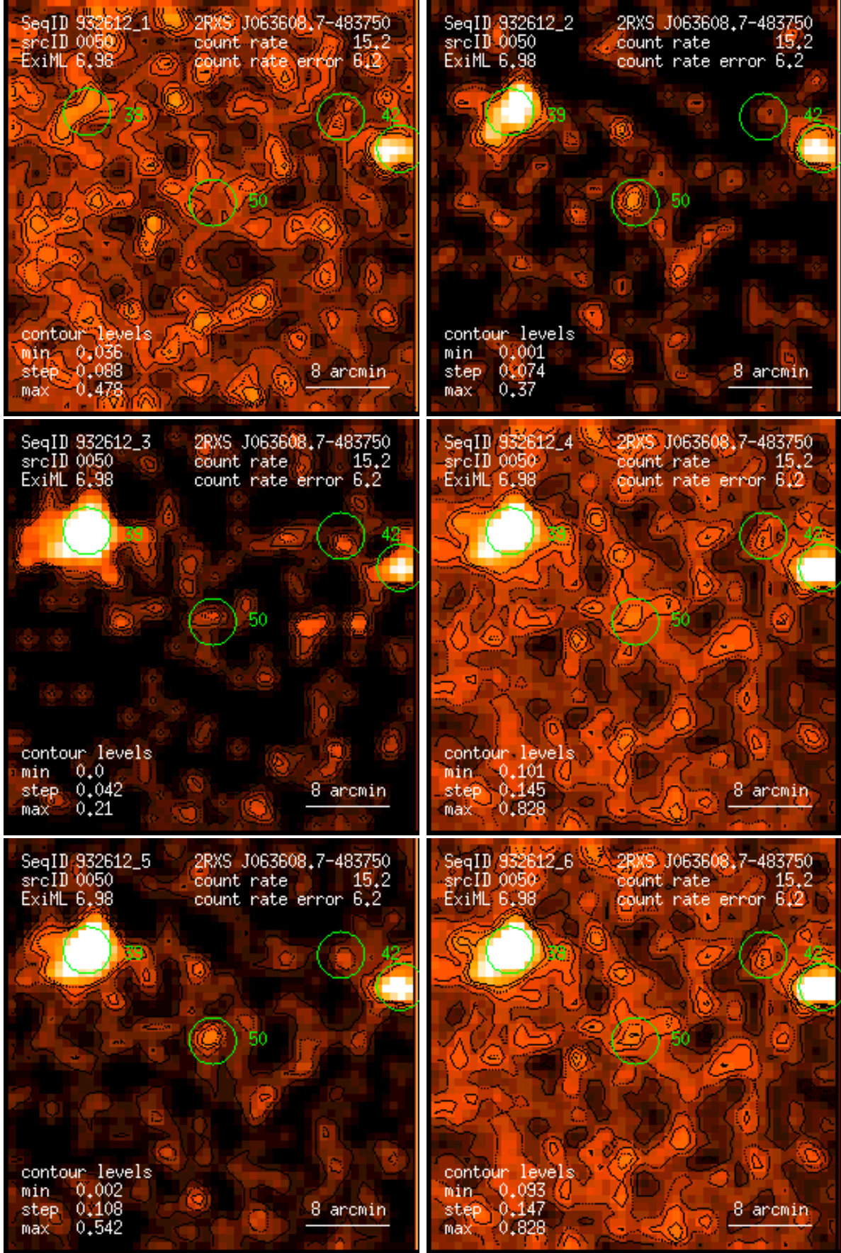
Figure 50: RASS 932612: detection 0050: band rate images, Gaussian filter: (1) PSPC channels 11 – 41, (2) 52 – 90, (3) 91 – 201, (4) 11 – 235, (5) 52 – 201, (6) 11 – 201. Broad band rates in counts/ks. Band rate contour levels in counts/ks/arcmin 2 .
