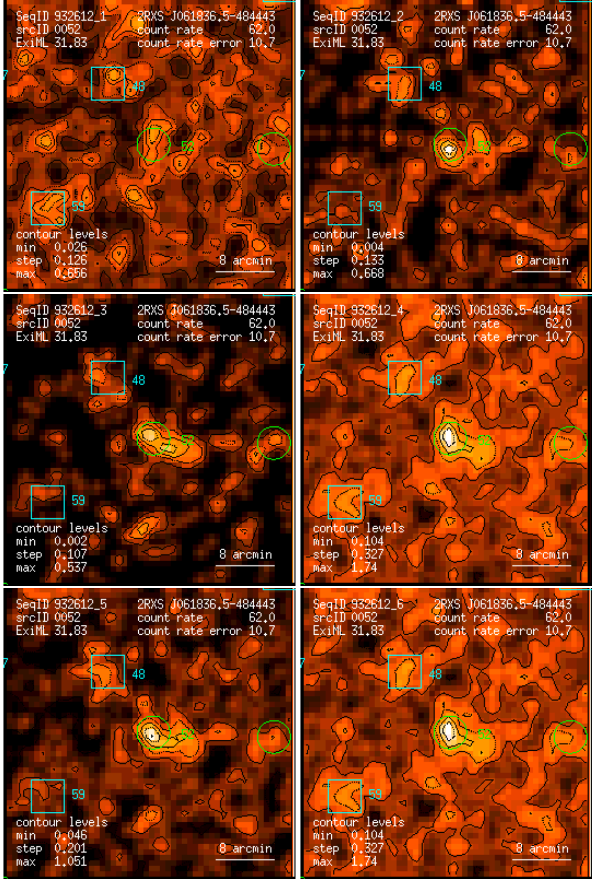
Figure 52: RASS 932612: detection 0052: band rate images, Gaussian filter: (1) PSPC channels 11 – 41, (2) 52 – 90, (3) 91 – 201, (4) 11 – 235, (5) 52 – 201, (6) 11 – 201. Broad band rates in counts/ks. Band rate contour levels in counts/ks/arcmin 2 .
