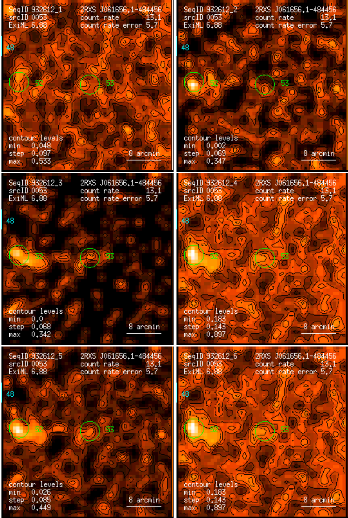
Figure 53: RASS 932612: detection 0053: band rate images, Gaussian filter: (1) PSPC channels 11 – 41, (2) 52 – 90, (3) 91 – 201, (4) 11 – 235, (5) 52 – 201, (6) 11 – 201. Broad band rates in counts/ks. Band rate contour levels in counts/ks/arcmin 2 .
