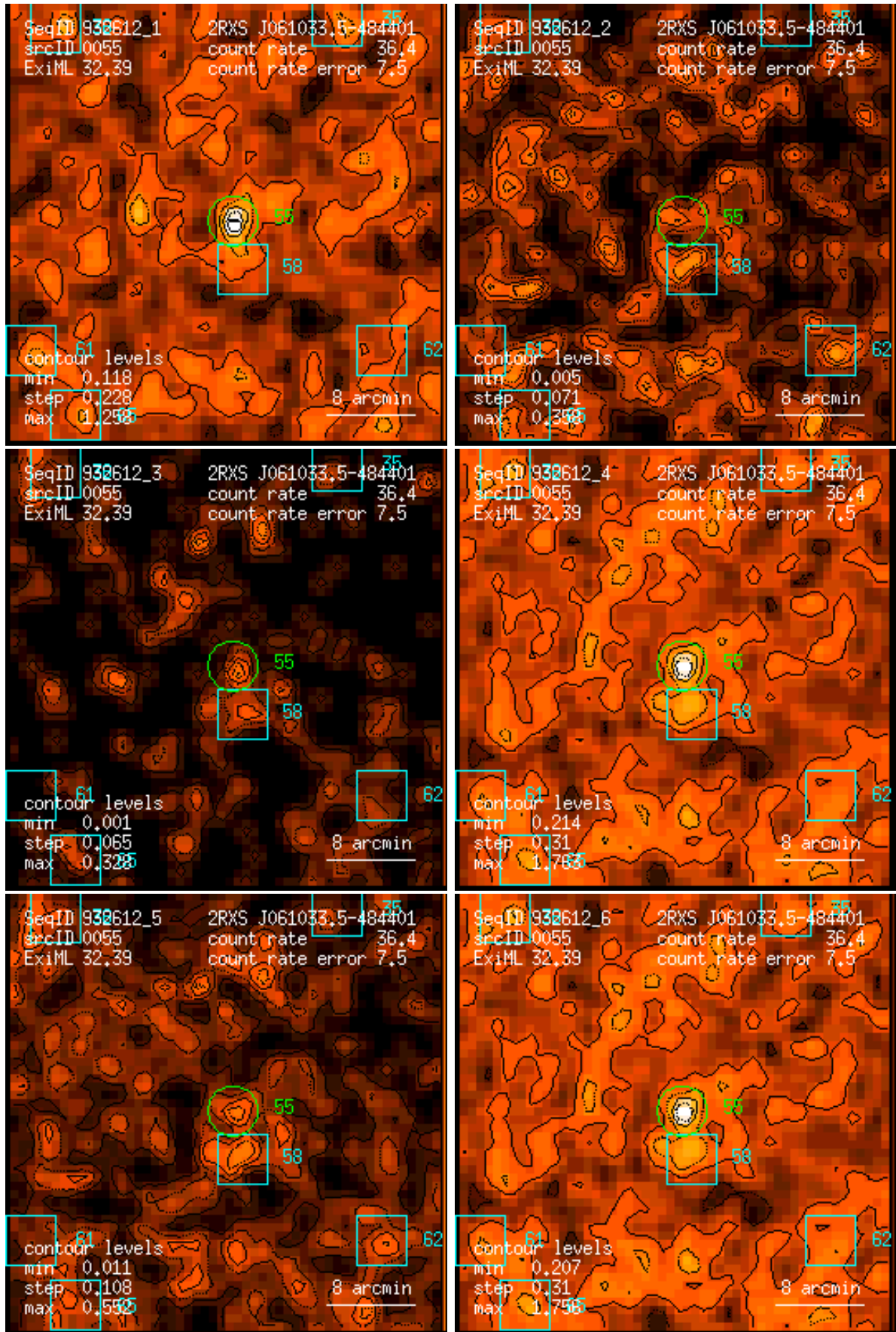
Figure 55: RASS 932612: detection 0055: band rate images, Gaussian filter: (1) PSPC channels 11 – 41, (2) 52 – 90, (3) 91 – 201, (4) 11 – 235, (5) 52 – 201, (6) 11 – 201. Broad band rates in counts/ks. Band rate contour levels in counts/ks/arcmin 2 .
