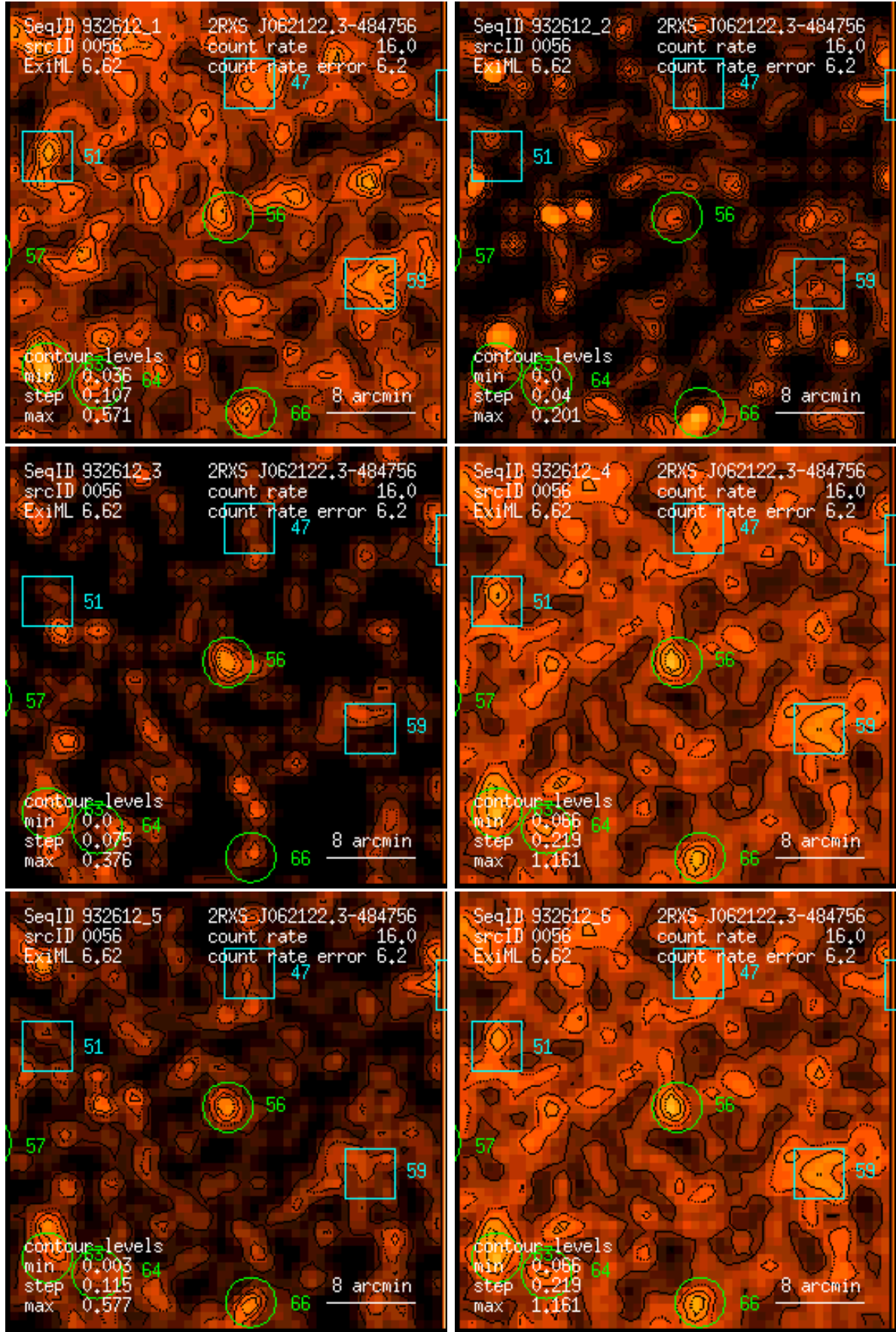
Figure 56: RASS 932612: detection 0056: band rate images, Gaussian filter: (1) PSPC channels 11 – 41, (2) 52 – 90, (3) 91 – 201, (4) 11 – 235, (5) 52 – 201, (6) 11 – 201. Broad band rates in counts/ks. Band rate contour levels in counts/ks/arcmin 2 .
