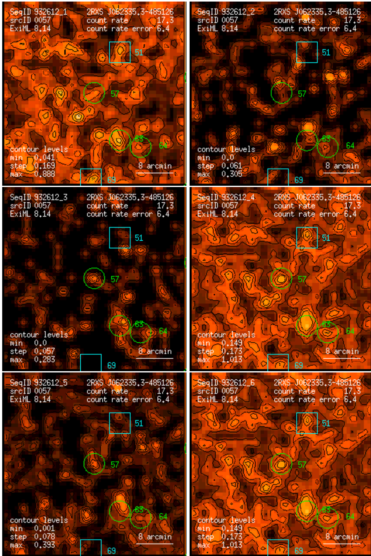
Figure 57: RASS 932612: detection 0057: band rate images, Gaussian filter: (1) PSPC channels 11 – 41, (2) 52 – 90, (3) 91 – 201, (4) 11 – 235, (5) 52 – 201, (6) 11 – 201. Broad band rates in counts/ks. Band rate contour levels in counts/ks/arcmin 2 .
