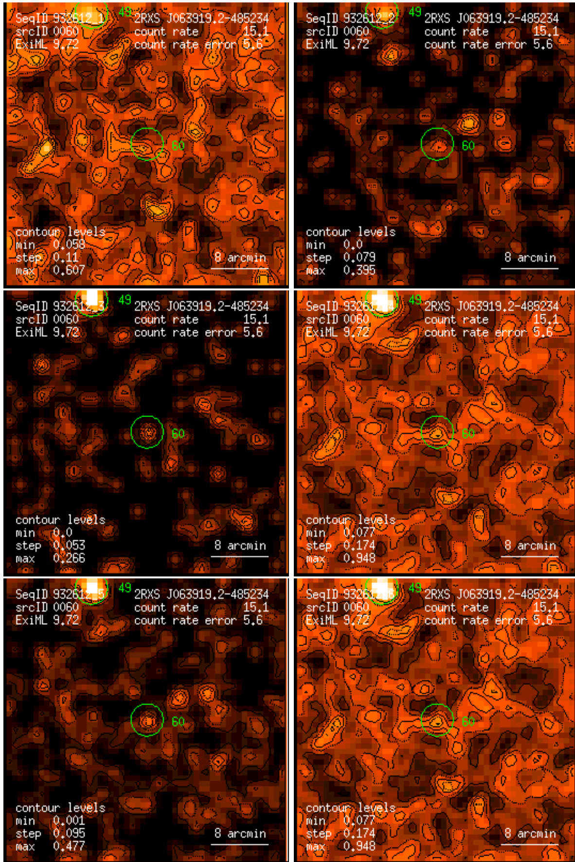
Figure 60: RASS 932612: detection 0060: band rate images, Gaussian filter: (1) PSPC channels 11 – 41, (2) 52 – 90, (3) 91 – 201, (4) 11 – 235, (5) 52 – 201, (6) 11 – 201. Broad band rates in counts/ks. Band rate contour levels in counts/ks/arcmin 2 .
