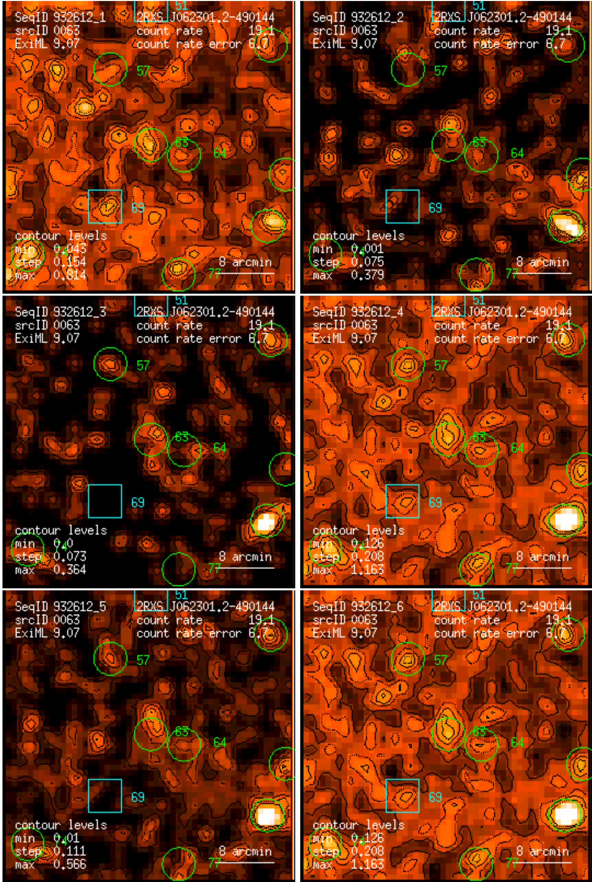
Figure 63: RASS 932612: detection 0063: band rate images, Gaussian filter: (1) PSPC channels 11 – 41, (2) 52 – 90, (3) 91 – 201, (4) 11 – 235, (5) 52 – 201, (6) 11 – 201. Broad band rates in counts/ks. Band rate contour levels in counts/ks/arcmin 2 .
