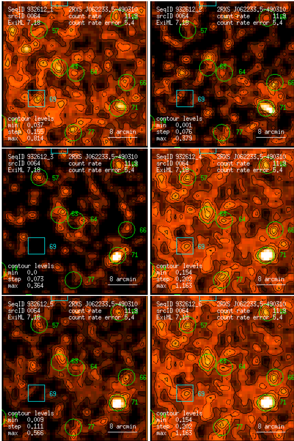
Figure 64: RASS 932612: detection 0064: band rate images, Gaussian filter: (1) PSPC channels 11 – 41, (2) 52 – 90, (3) 91 – 201, (4) 11 – 235, (5) 52 – 201, (6) 11 – 201. Broad band rates in counts/ks. Band rate contour levels in counts/ks/arcmin 2 .
