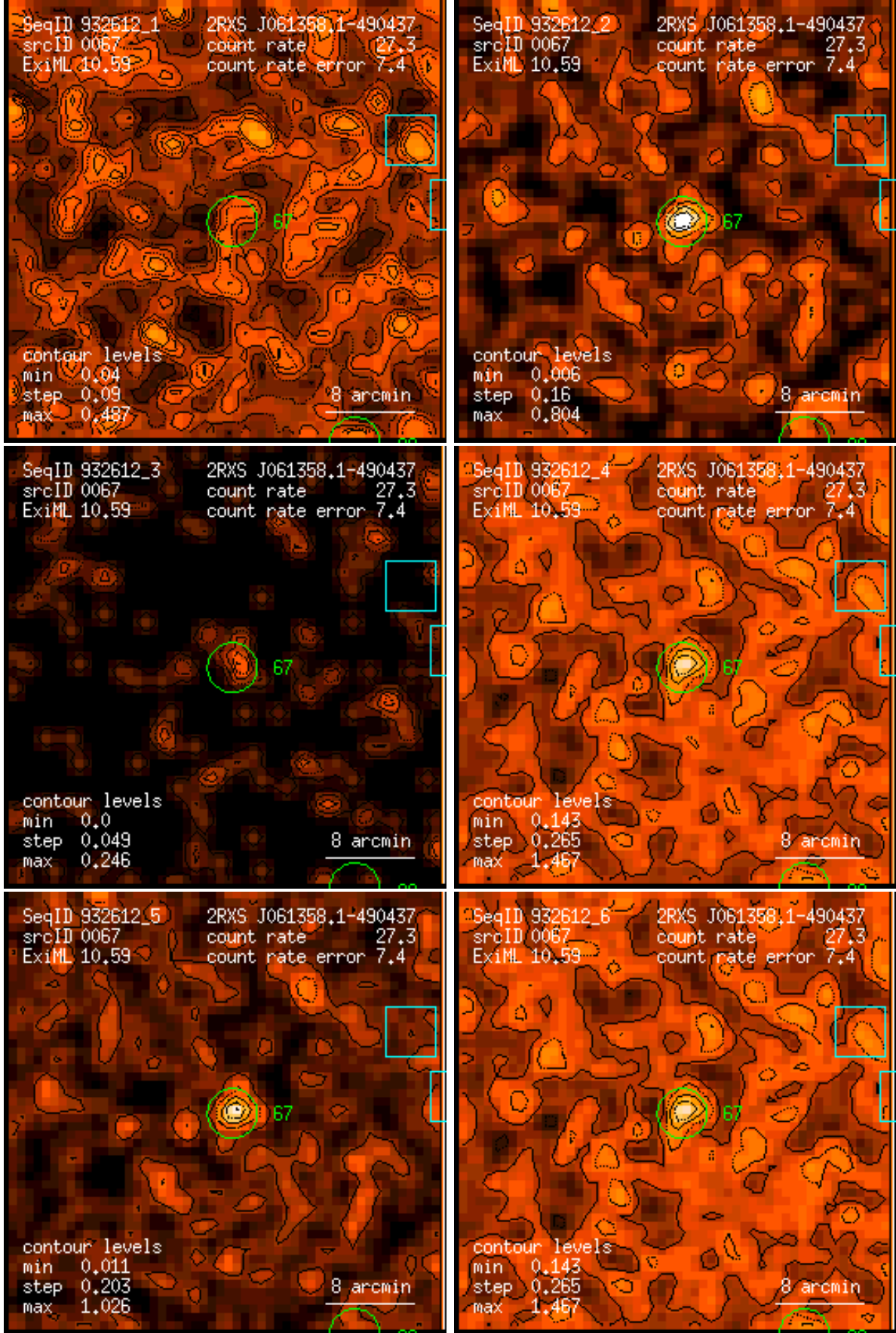
Figure 67: RASS 932612: detection 0067: band rate images, Gaussian filter: (1) PSPC channels 11 – 41, (2) 52 – 90, (3) 91 – 201, (4) 11 – 235, (5) 52 – 201, (6) 11 – 201. Broad band rates in counts/ks. Band rate contour levels in counts/ks/arcmin 2 .
