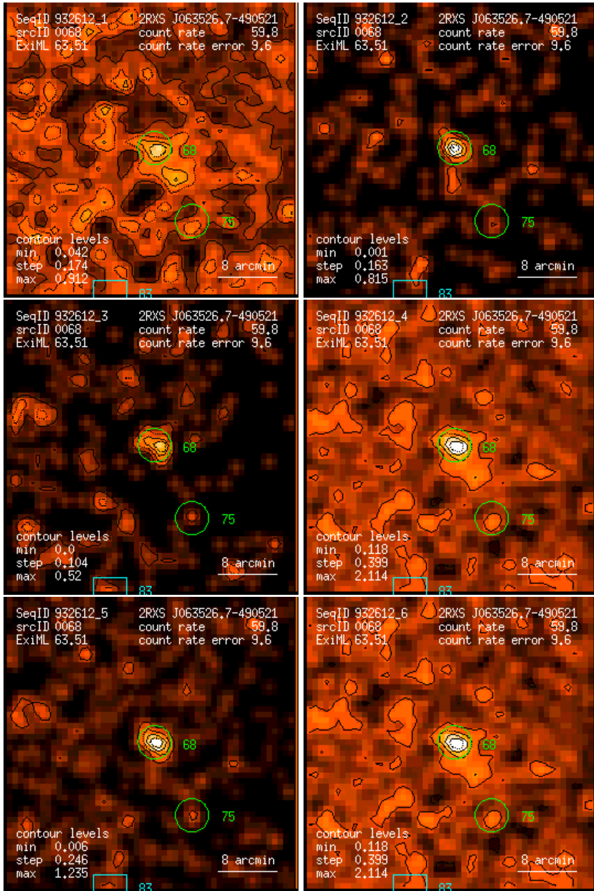
Figure 68: RASS 932612: detection 0068: band rate images, Gaussian filter: (1) PSPC channels 11 – 41, (2) 52 – 90, (3) 91 – 201, (4) 11 – 235, (5) 52 – 201, (6) 11 – 201. Broad band rates in counts/ks. Band rate contour levels in counts/ks/arcmin 2 .
