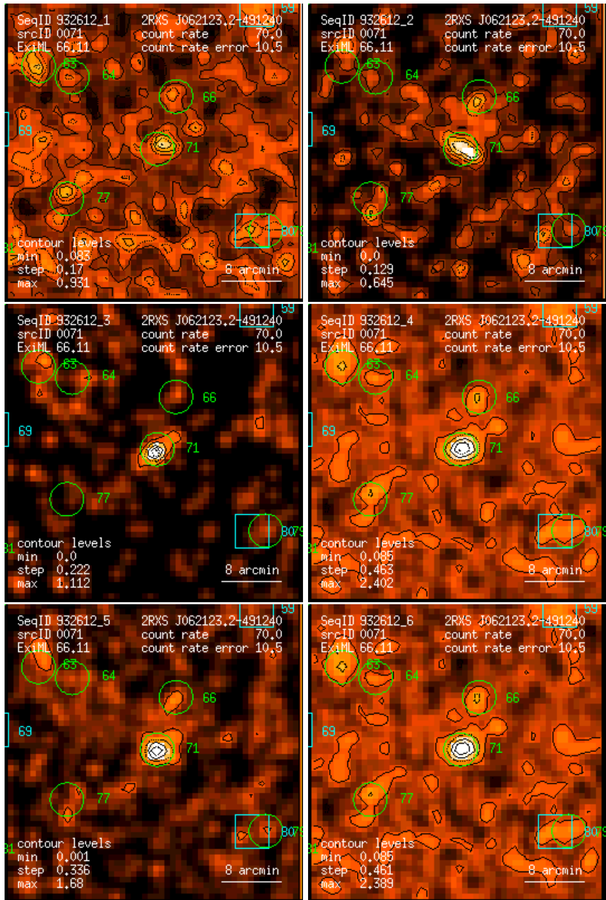
Figure 71: RASS 932612: detection 0071: band rate images, Gaussian filter: (1) PSPC channels 11 – 41, (2) 52 – 90, (3) 91 – 201, (4) 11 – 235, (5) 52 – 201, (6) 11 – 201. Broad band rates in counts/ks. Band rate contour levels in counts/ks/arcmin 2 .
