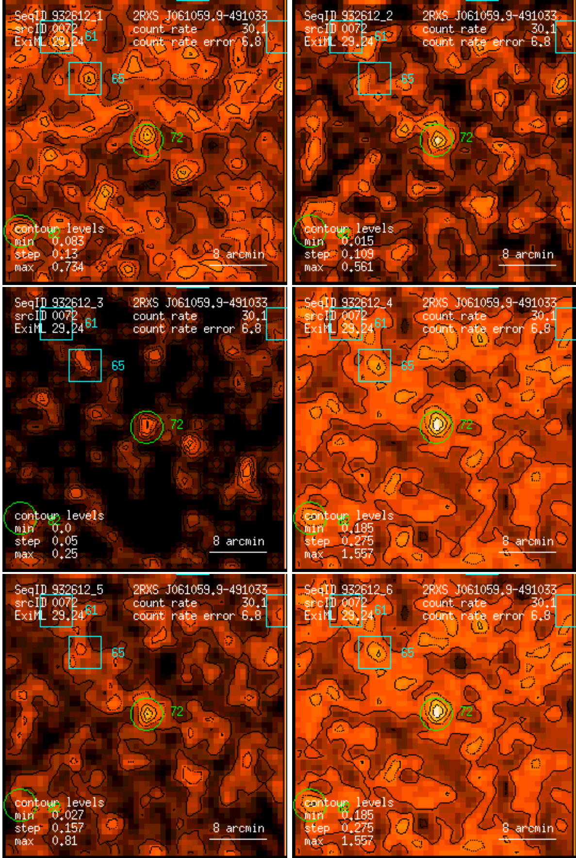
Figure 72: RASS 932612: detection 0072: band rate images, Gaussian filter: (1) PSPC channels 11 – 41, (2) 52 – 90, (3) 91 – 201, (4) 11 – 235, (5) 52 – 201, (6) 11 – 201. Broad band rates in counts/ks. Band rate contour levels in counts/ks/arcmin 2 .
