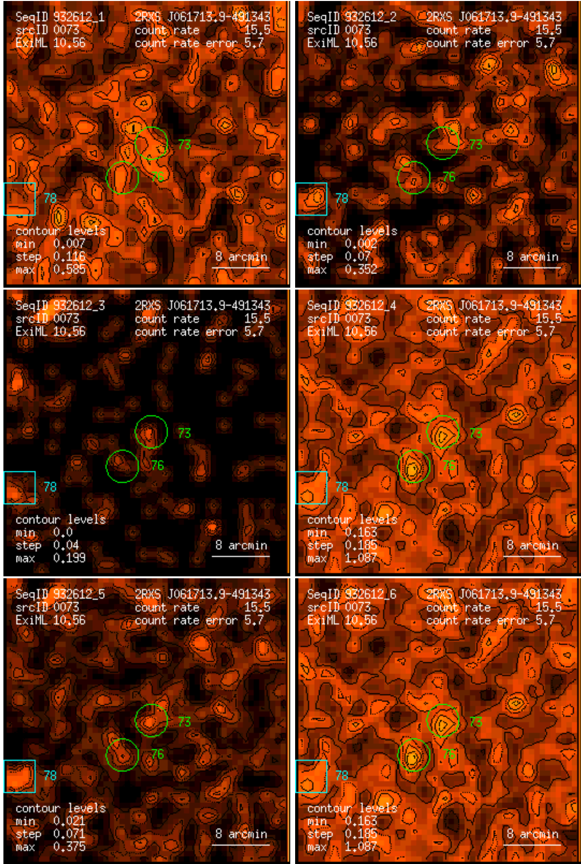
Figure 73: RASS 932612: detection 0073: band rate images, Gaussian filter: (1) PSPC channels 11 – 41, (2) 52 – 90, (3) 91 – 201, (4) 11 – 235, (5) 52 – 201, (6) 11 – 201. Broad band rates in counts/ks. Band rate contour levels in counts/ks/arcmin 2 .
