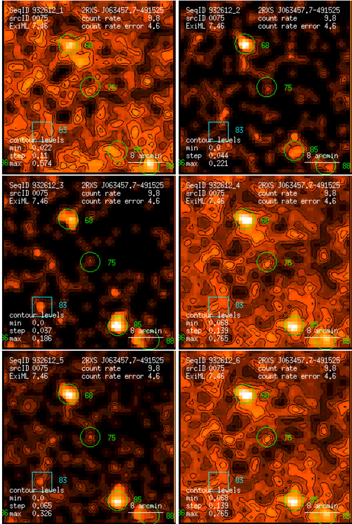
Figure 75: RASS 932612: detection 0075: band rate images, Gaussian filter: (1) PSPC channels 11 – 41, (2) 52 – 90, (3) 91 – 201, (4) 11 – 235, (5) 52 – 201, (6) 11 – 201. Broad band rates in counts/ks. Band rate contour levels in counts/ks/arcmin 2 .
