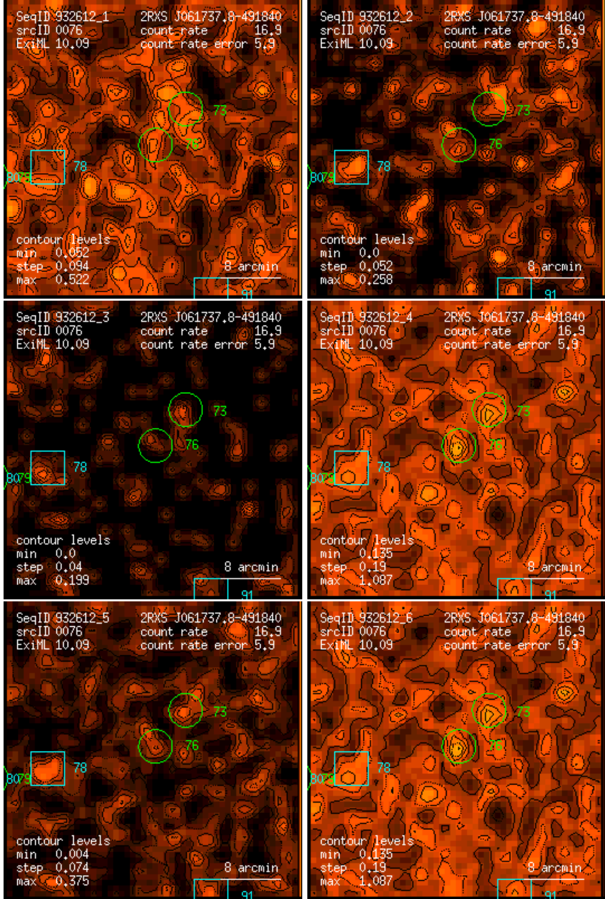
Figure 76: RASS 932612: detection 0076: band rate images, Gaussian filter: (1) PSPC channels 11 – 41, (2) 52 – 90, (3) 91 – 201, (4) 11 – 235, (5) 52 – 201, (6) 11 – 201. Broad band rates in counts/ks. Band rate contour levels in counts/ks/arcmin 2 .
