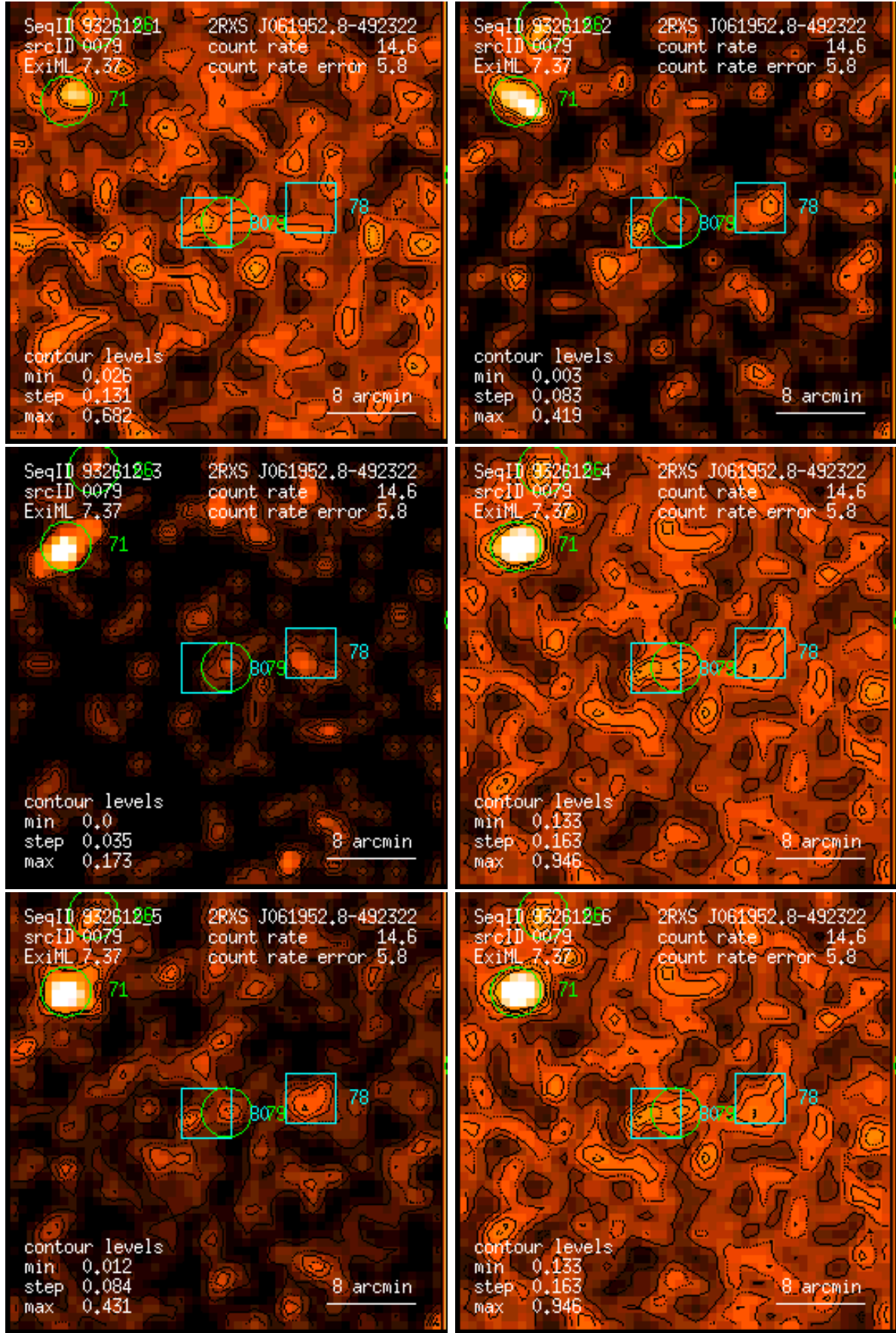
Figure 79: RASS 932612: detection 0079: band rate images, Gaussian filter: (1) PSPC channels 11 – 41, (2) 52 – 90, (3) 91 – 201, (4) 11 – 235, (5) 52 – 201, (6) 11 – 201. Broad band rates in counts/ks. Band rate contour levels in counts/ks/arcmin 2 .
