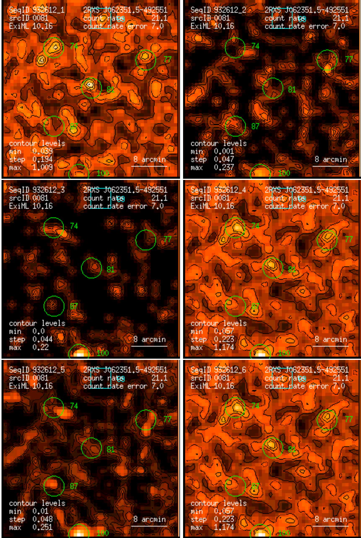
Figure 81: RASS 932612: detection 0081: band rate images, Gaussian filter: (1) PSPC channels 11 – 41, (2) 52 – 90, (3) 91 – 201, (4) 11 – 235, (5) 52 – 201, (6) 11 – 201. Broad band rates in counts/ks. Band rate contour levels in counts/ks/arcmin 2 .
