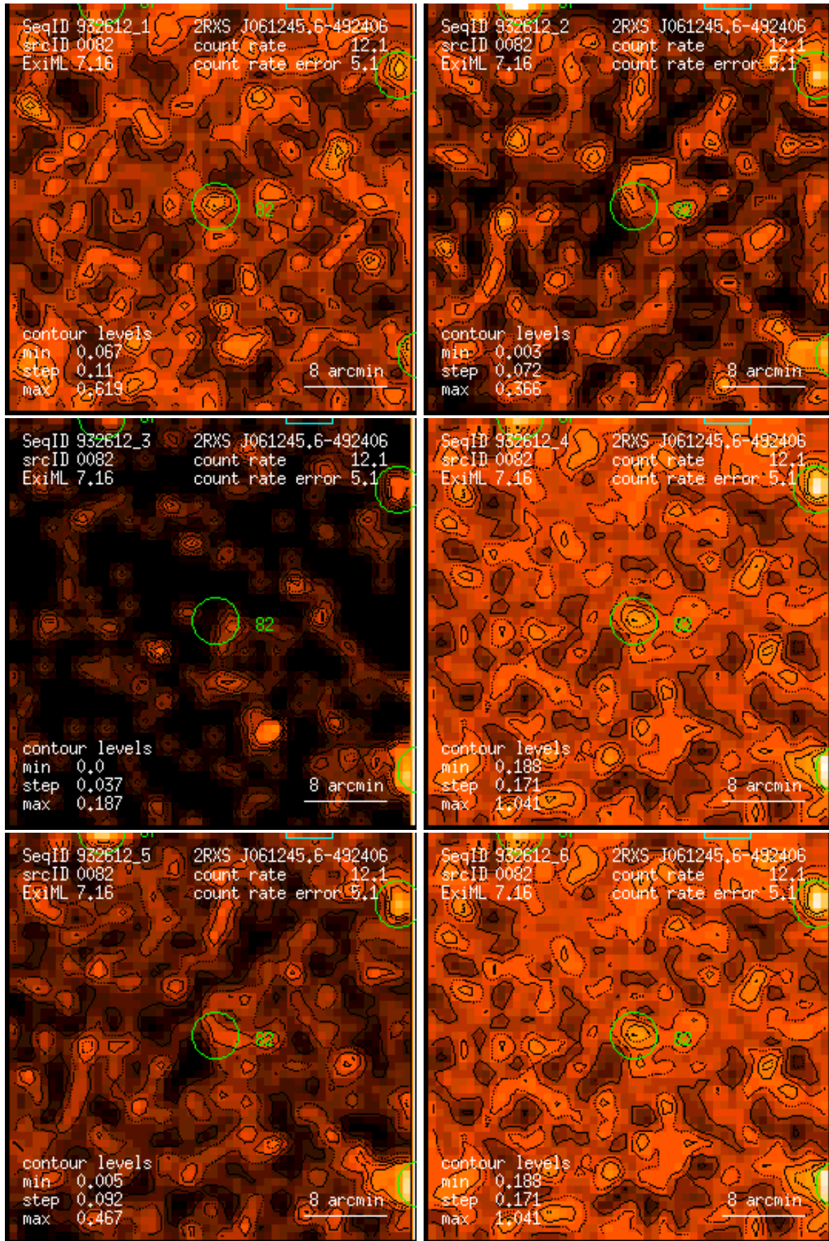
Figure 82: RASS 932612: detection 0082: band rate images, Gaussian filter: (1) PSPC channels 11 – 41, (2) 52 – 90, (3) 91 – 201, (4) 11 – 235, (5) 52 – 201, (6) 11 – 201. Broad band rates in counts/ks. Band rate contour levels in counts/ks/arcmin 2 .
