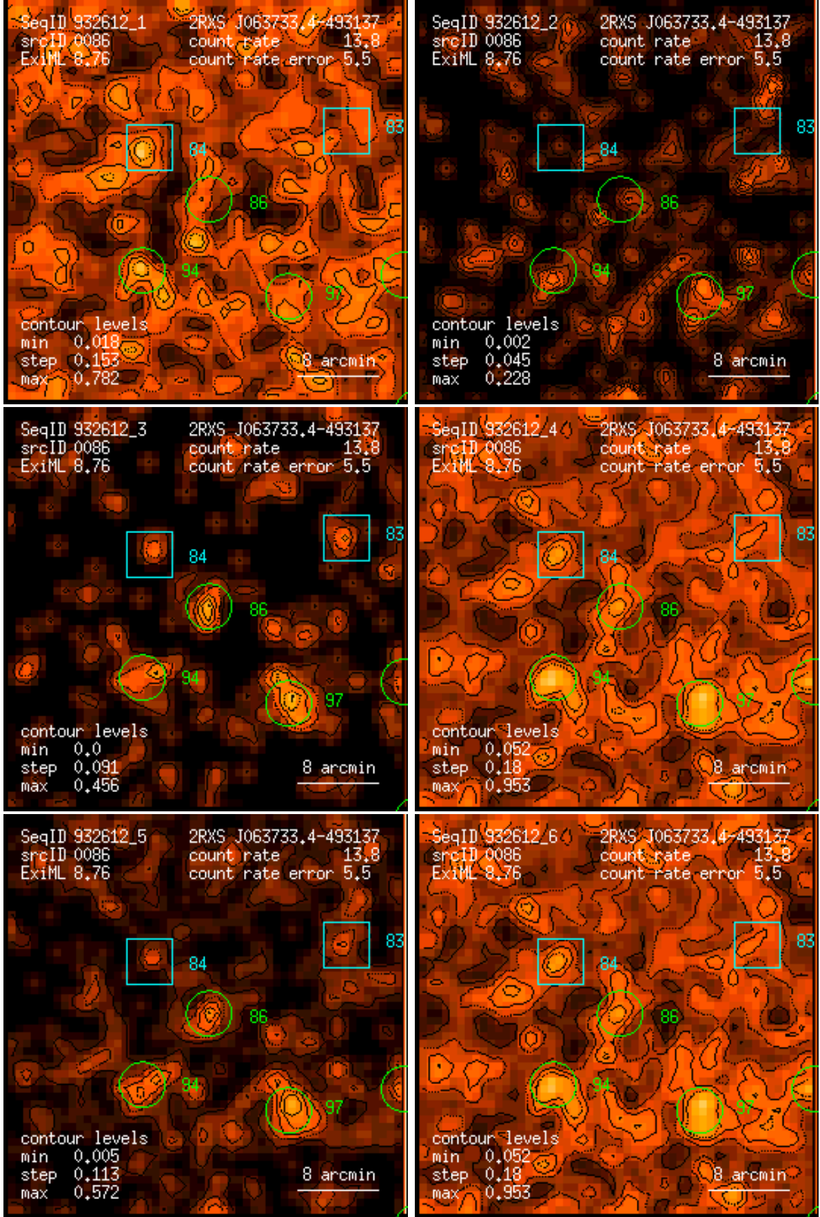
Figure 86: RASS 932612: detection 0086: band rate images, Gaussian filter: (1) PSPC channels 11 – 41, (2) 52 – 90, (3) 91 – 201, (4) 11 – 235, (5) 52 – 201, (6) 11 – 201. Broad band rates in counts/ks. Band rate contour levels in counts/ks/arcmin 2 .
