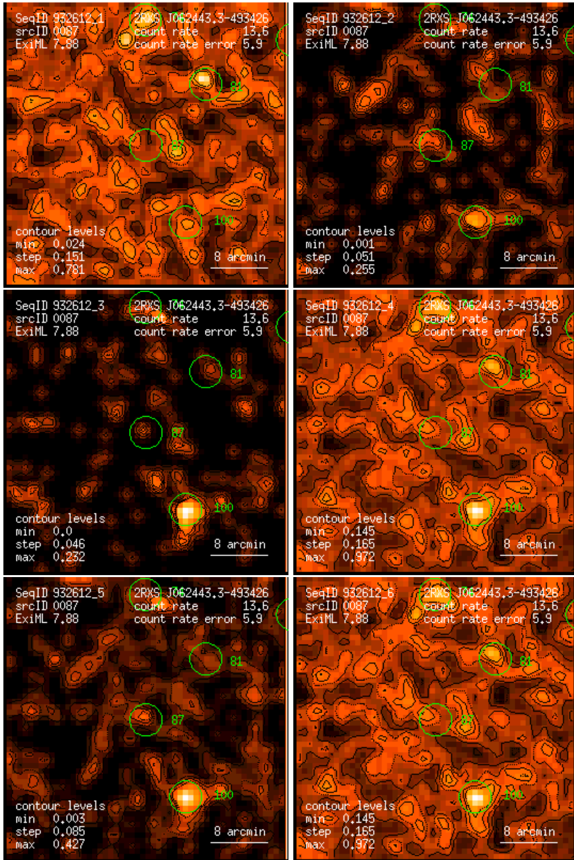
Figure 87: RASS 932612: detection 0087: band rate images, Gaussian filter: (1) PSPC channels 11 – 41, (2) 52 – 90, (3) 91 – 201, (4) 11 – 235, (5) 52 – 201, (6) 11 – 201. Broad band rates in counts/ks. Band rate contour levels in counts/ks/arcmin 2 .
