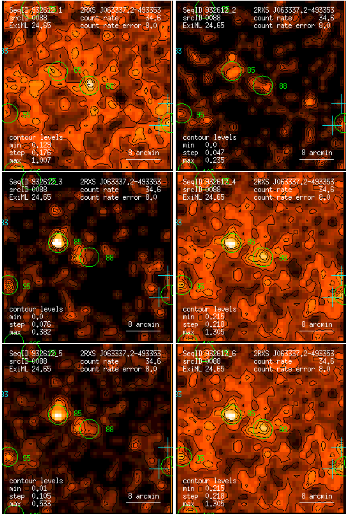
Figure 88: RASS 932612: detection 0088: band rate images, Gaussian filter: (1) PSPC channels 11 – 41, (2) 52 – 90, (3) 91 – 201, (4) 11 – 235, (5) 52 – 201, (6) 11 – 201. Broad band rates in counts/ks. Band rate contour levels in counts/ks/arcmin 2 .
