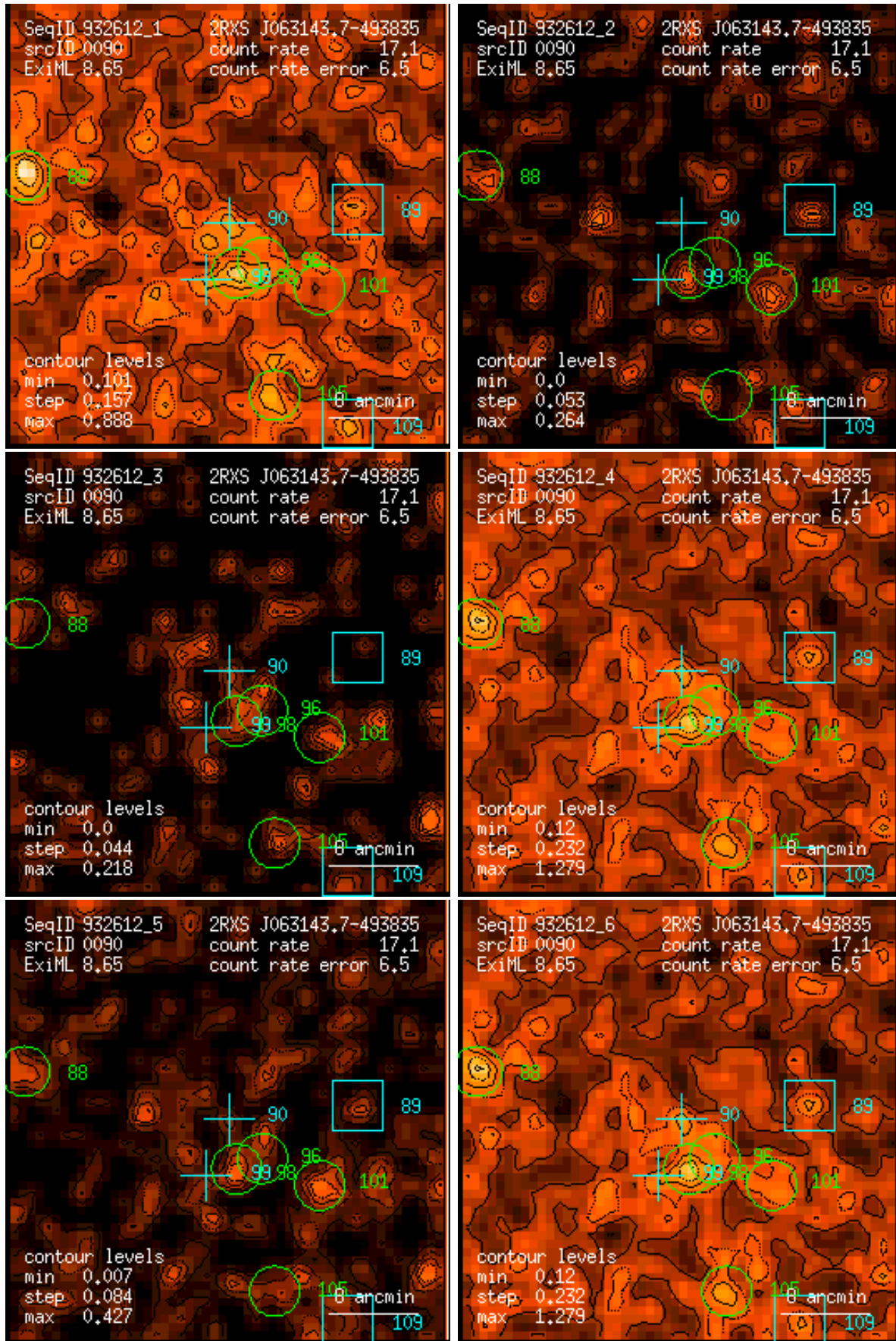
Figure 90: RASS 932612: detection 0090: band rate images, Gaussian filter: (1) PSPC channels 11 – 41, (2) 52 – 90, (3) 91 – 201, (4) 11 – 235, (5) 52 – 201, (6) 11 – 201. Broad band rates in counts/ks. Band rate contour levels in counts/ks/arcmin 2 .
