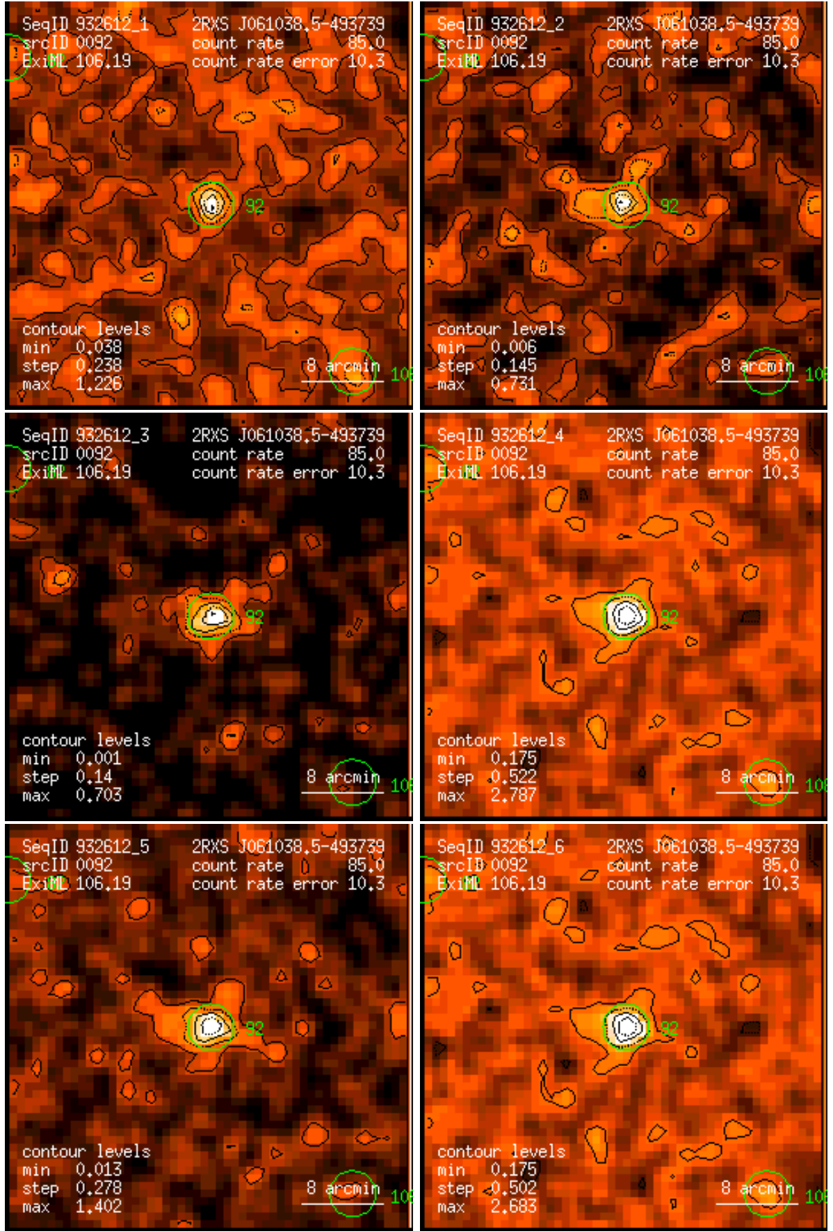
Figure 92: RASS 932612: detection 0092: band rate images, Gaussian filter: (1) PSPC channels 11 – 41, (2) 52 – 90, (3) 91 – 201, (4) 11 – 235, (5) 52 – 201, (6) 11 – 201. Broad band rates in counts/ks. Band rate contour levels in counts/ks/arcmin 2 .
