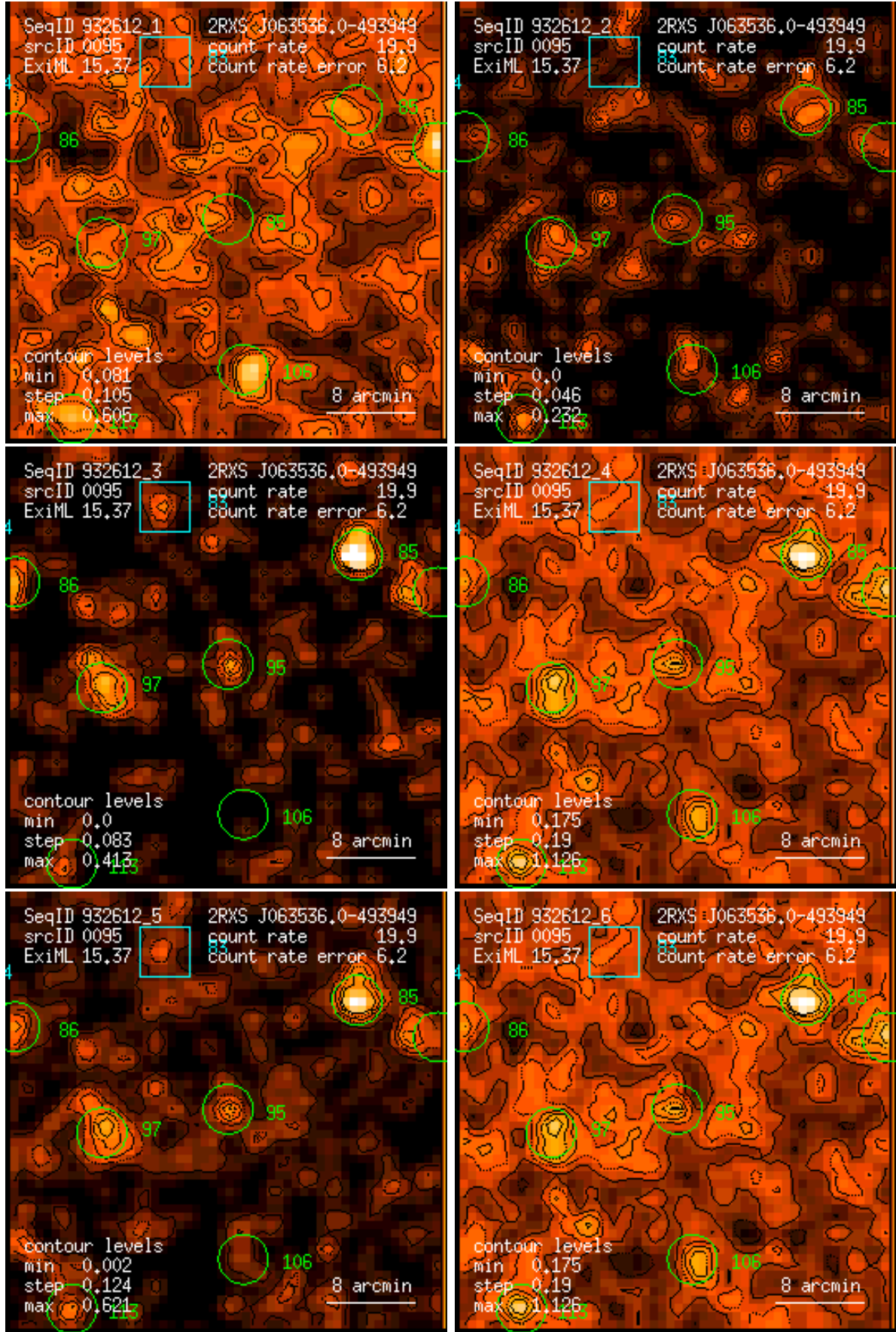
Figure 95: RASS 932612: detection 0095: band rate images, Gaussian filter: (1) PSPC channels 11 – 41, (2) 52 – 90, (3) 91 – 201, (4) 11 – 235, (5) 52 – 201, (6) 11 – 201. Broad band rates in counts/ks. Band rate contour levels in counts/ks/arcmin 2 .
